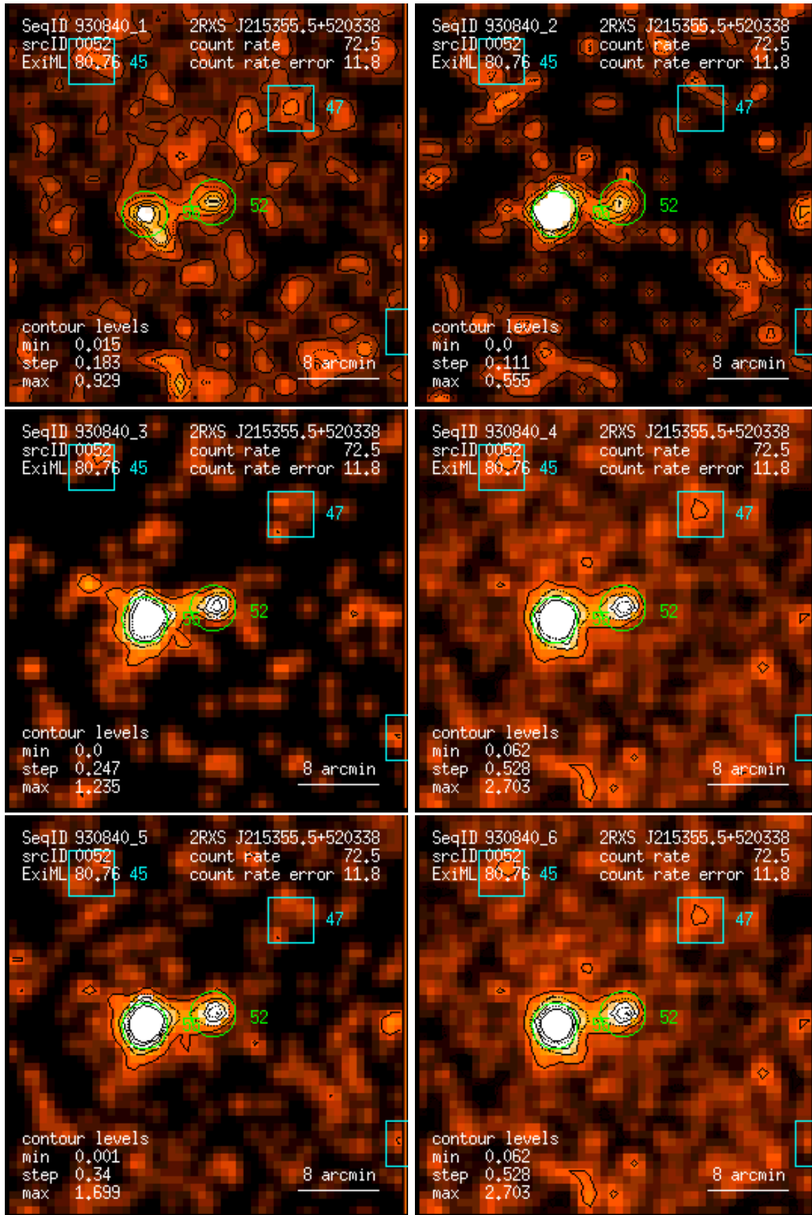
Figure 52: RASS 930840: detection 0052: band rate images, Gaussian filter: (1) PSPC channels 11 – 41, (2) 52 – 90, (3) 91 – 201, (4) 11 – 235, (5) 52 – 201, (6) 11 – 201. Broad band rates in counts/ks. Band rate contour levels in counts/ks/arcmin 2 .
