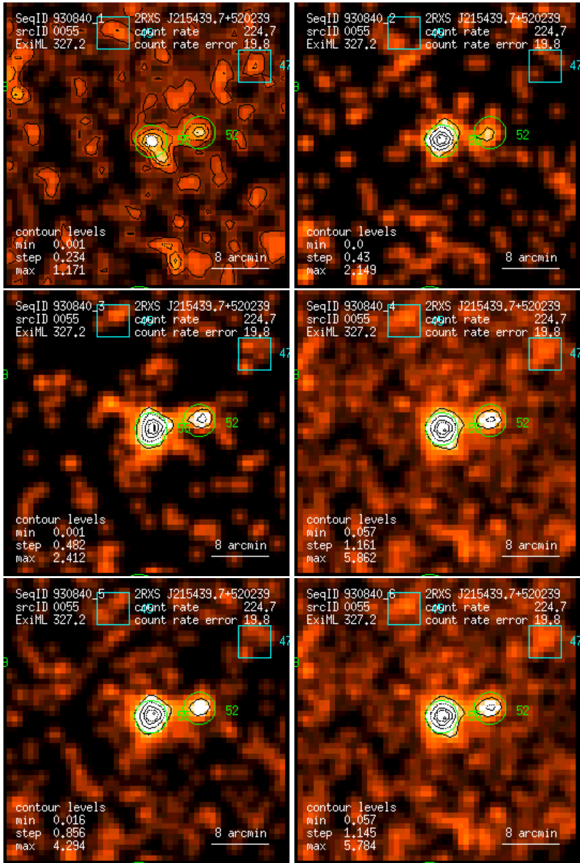
Figure 55: RASS 930840: detection 0055: band rate images, Gaussian filter: (1) PSPC channels 11 – 41, (2) 52 – 90, (3) 91 – 201, (4) 11 – 235, (5) 52 – 201, (6) 11 – 201. Broad band rates in counts/ks. Band rate contour levels in counts/ks/arcmin 2 .
