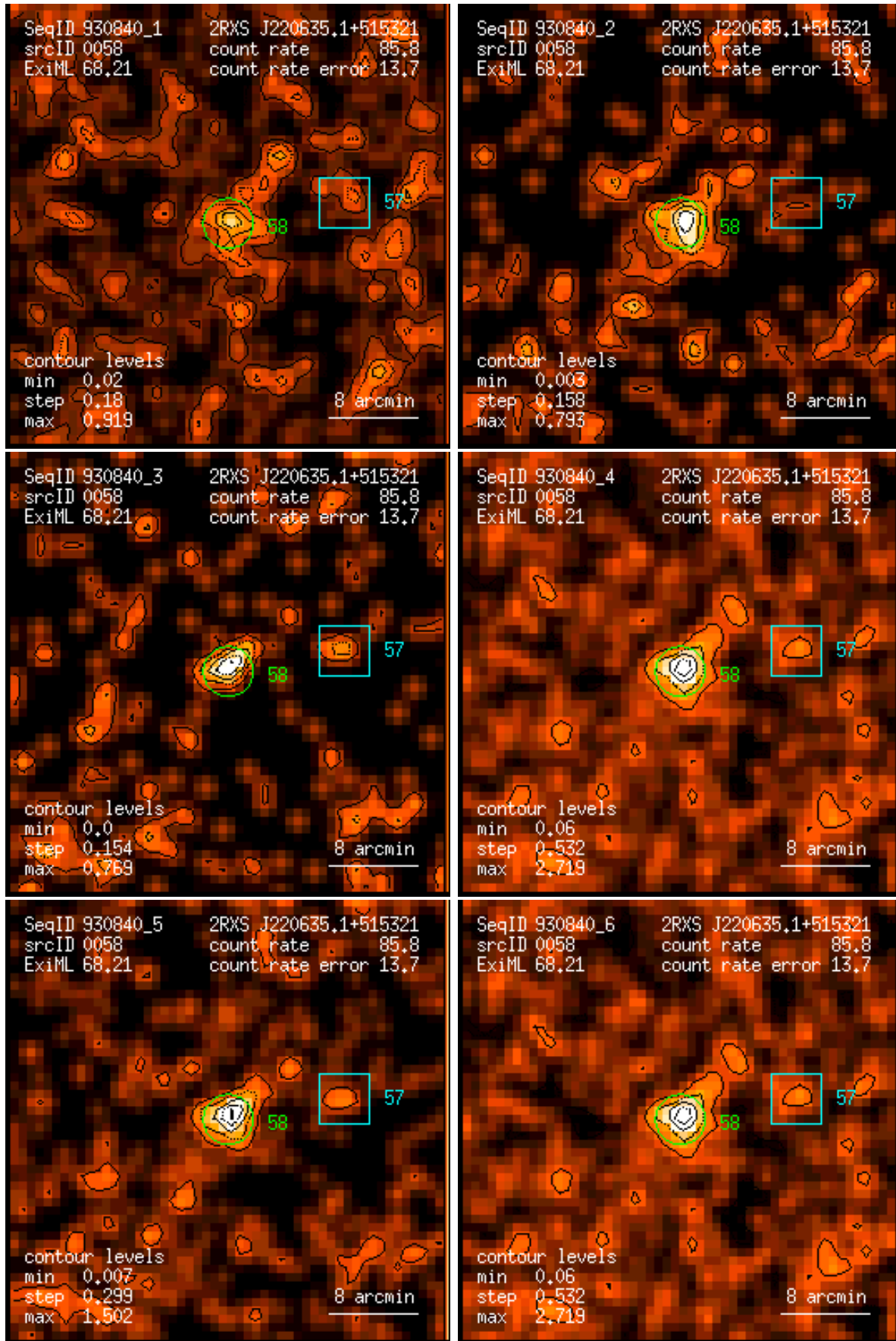
Figure 58: RASS 930840: detection 0058: band rate images, Gaussian filter: (1) PSPC channels 11 – 41, (2) 52 – 90, (3) 91 – 201, (4) 11 – 235, (5) 52 – 201, (6) 11 – 201. Broad band rates in counts/ks. Band rate contour levels in counts/ks/arcmin 2 .
