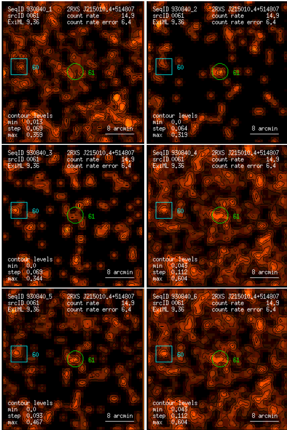
Figure 61: RASS 930840: detection 0061: band rate images, Gaussian filter: (1) PSPC channels 11 – 41, (2) 52 – 90, (3) 91 – 201, (4) 11 – 235, (5) 52 – 201, (6) 11 – 201. Broad band rates in counts/ks. Band rate contour levels in counts/ks/arcmin 2 .
