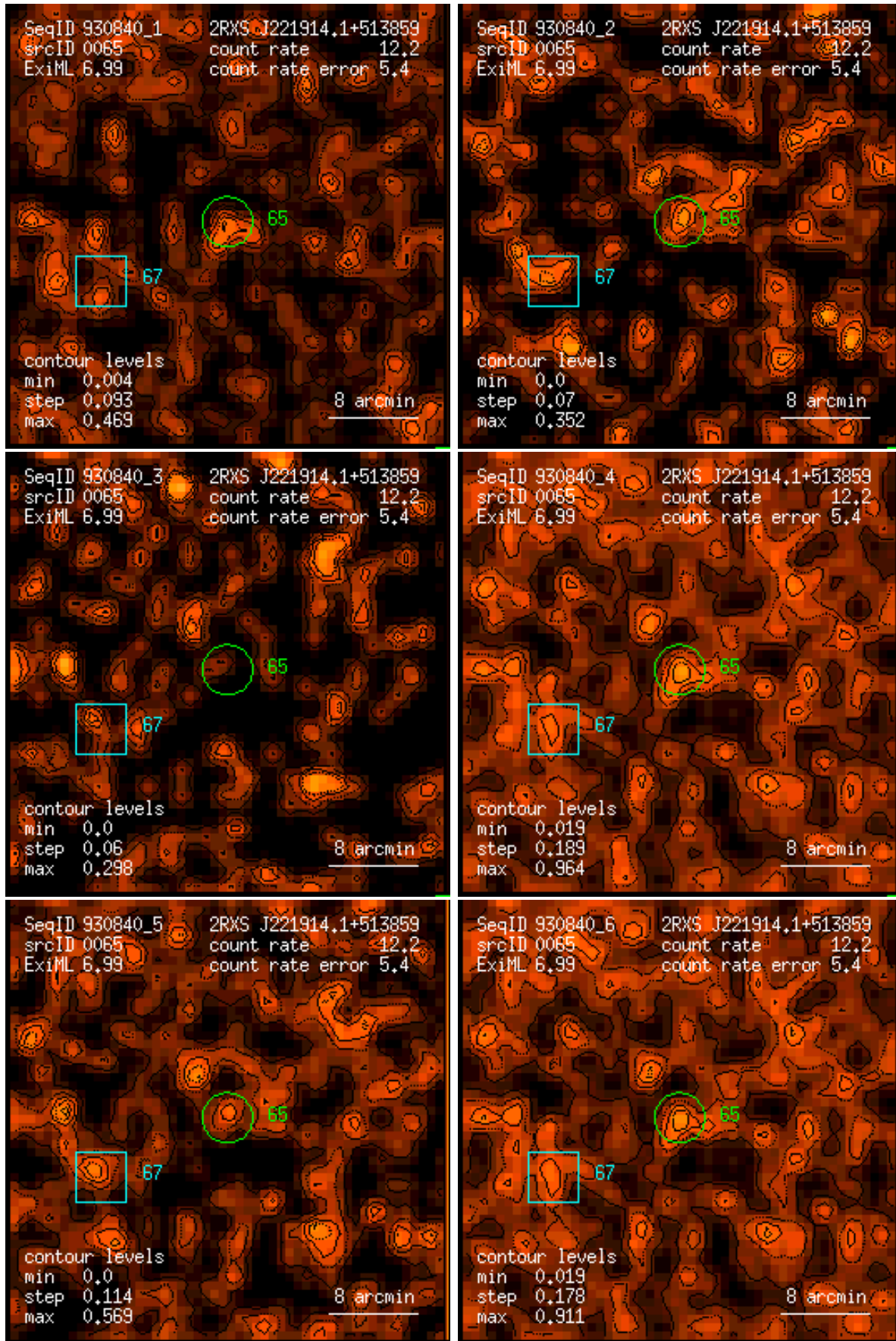
Figure 65: RASS 930840: detection 0065: band rate images, Gaussian filter: (1) PSPC channels 11 – 41, (2) 52 – 90, (3) 91 – 201, (4) 11 – 235, (5) 52 – 201, (6) 11 – 201. Broad band rates in counts/ks. Band rate contour levels in counts/ks/arcmin 2 .
