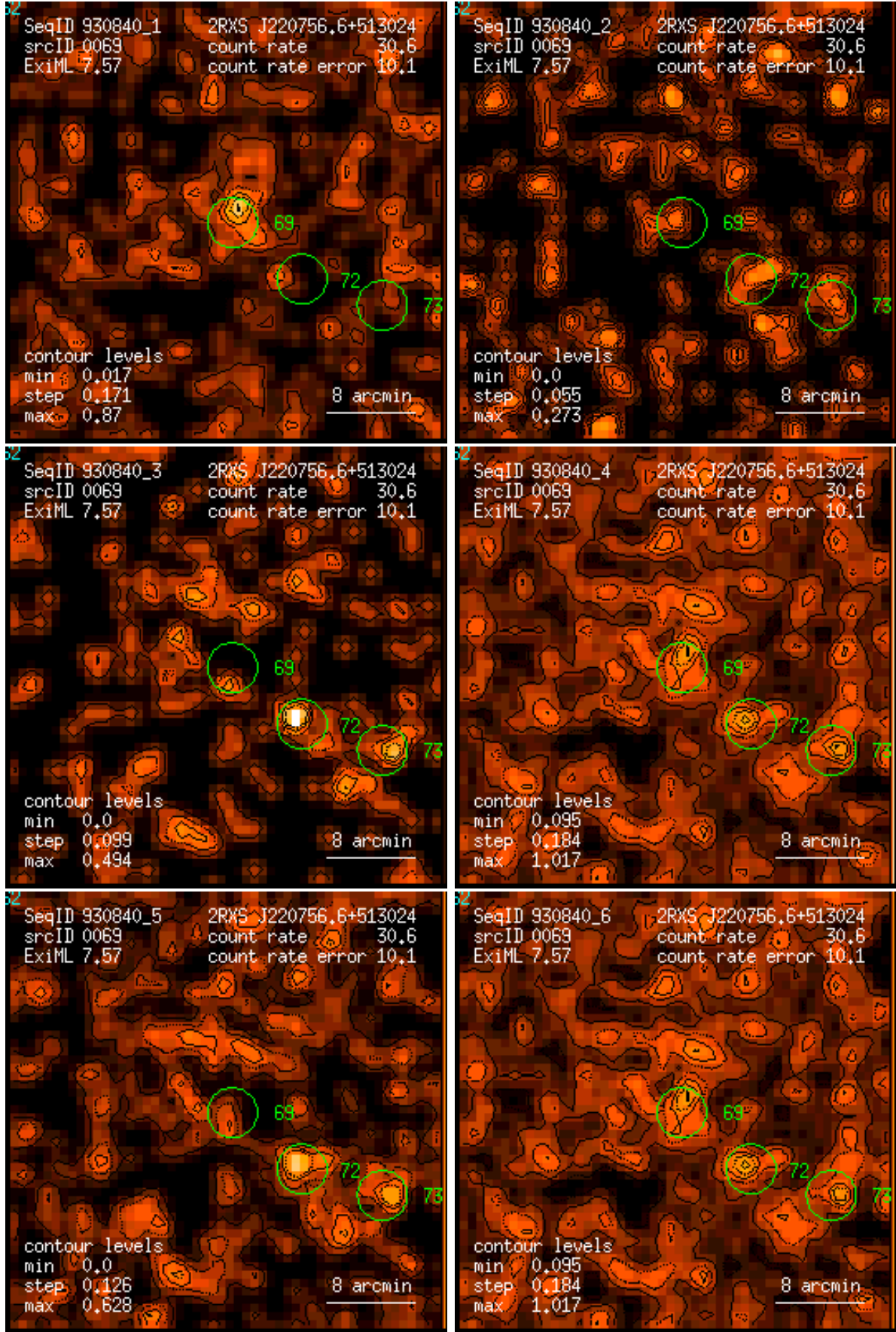
Figure 69: RASS 930840: detection 0069: band rate images, Gaussian filter: (1) PSPC channels 11 – 41, (2) 52 – 90, (3) 91 – 201, (4) 11 – 235, (5) 52 – 201, (6) 11 – 201. Broad band rates in counts/ks. Band rate contour levels in counts/ks/arcmin 2 .
