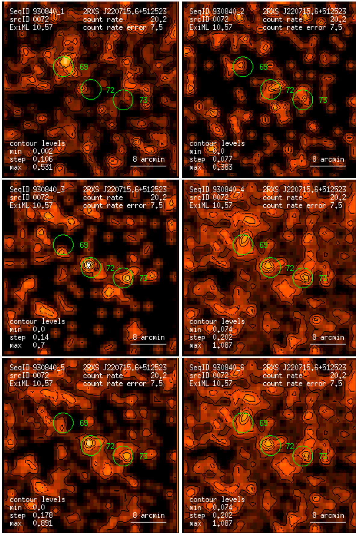
Figure 72: RASS 930840: detection 0072: band rate images, Gaussian filter: (1) PSPC channels 11 – 41, (2) 52 – 90, (3) 91 – 201, (4) 11 – 235, (5) 52 – 201, (6) 11 – 201. Broad band rates in counts/ks. Band rate contour levels in counts/ks/arcmin 2 .
