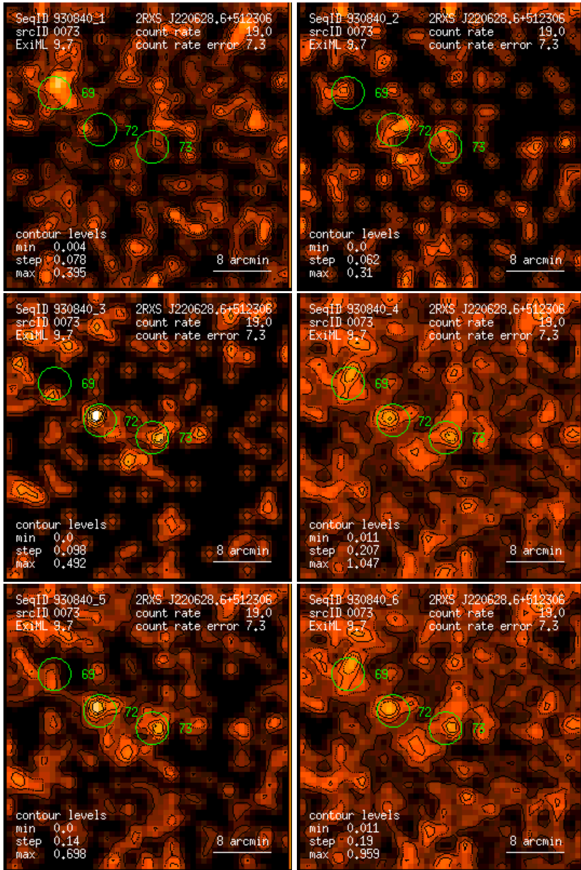
Figure 73: RASS 930840: detection 0073: band rate images, Gaussian filter: (1) PSPC channels 11 – 41, (2) 52 – 90, (3) 91 – 201, (4) 11 – 235, (5) 52 – 201, (6) 11 – 201. Broad band rates in counts/ks. Band rate contour levels in counts/ks/arcmin 2 .
