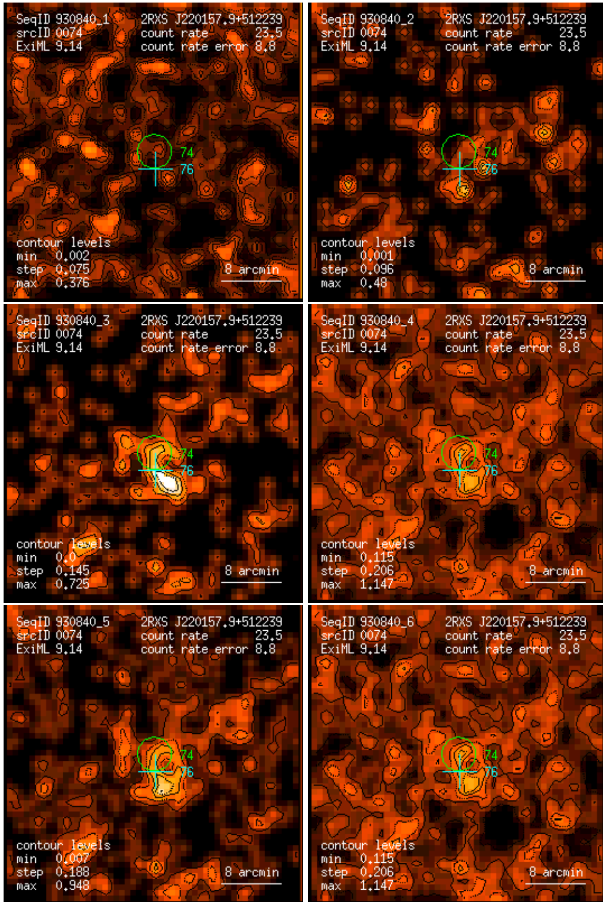
Figure 74: RASS 930840: detection 0074: band rate images, Gaussian filter: (1) PSPC channels 11 – 41, (2) 52 – 90, (3) 91 – 201, (4) 11 – 235, (5) 52 – 201, (6) 11 – 201. Broad band rates in counts/ks. Band rate contour levels in counts/ks/arcmin 2 .
