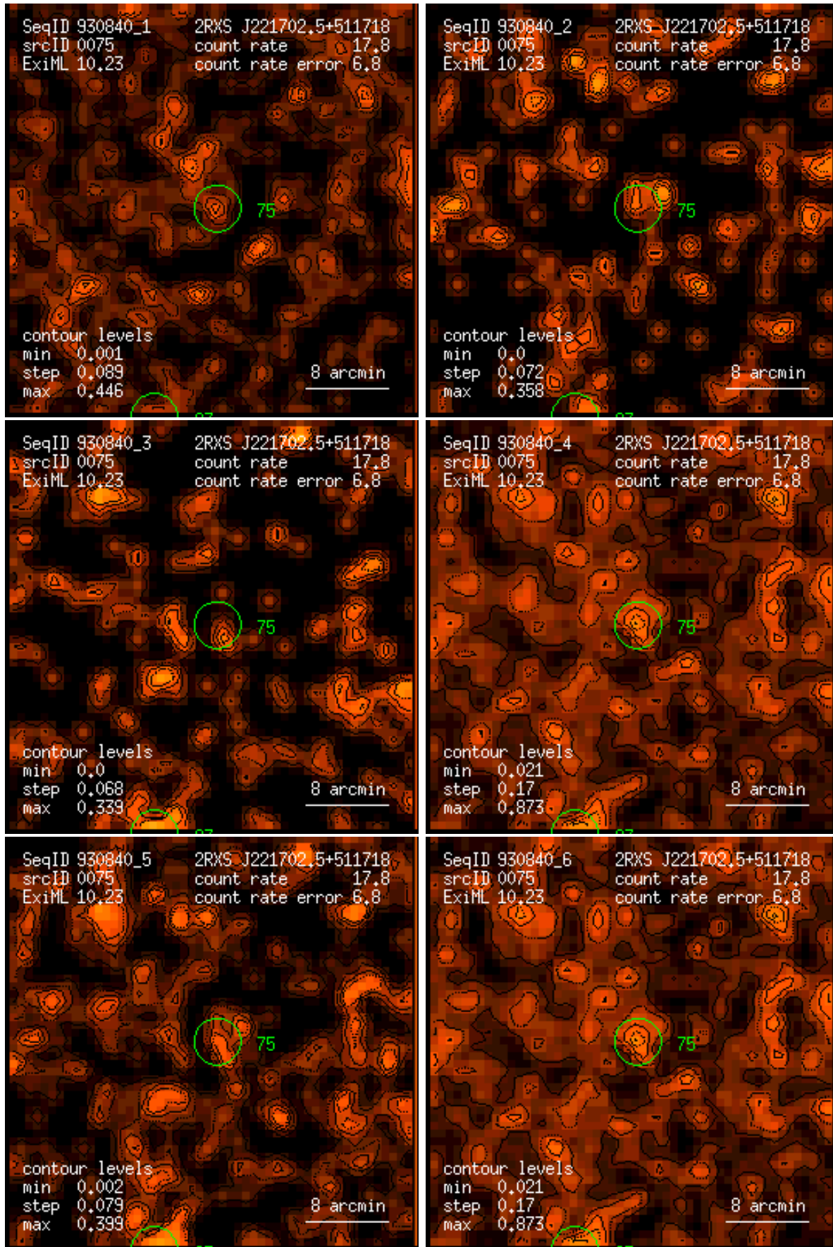
Figure 75: RASS 930840: detection 0075: band rate images, Gaussian filter: (1) PSPC channels 11 – 41, (2) 52 – 90, (3) 91 – 201, (4) 11 – 235, (5) 52 – 201, (6) 11 – 201. Broad band rates in counts/ks. Band rate contour levels in counts/ks/arcmin 2 .
