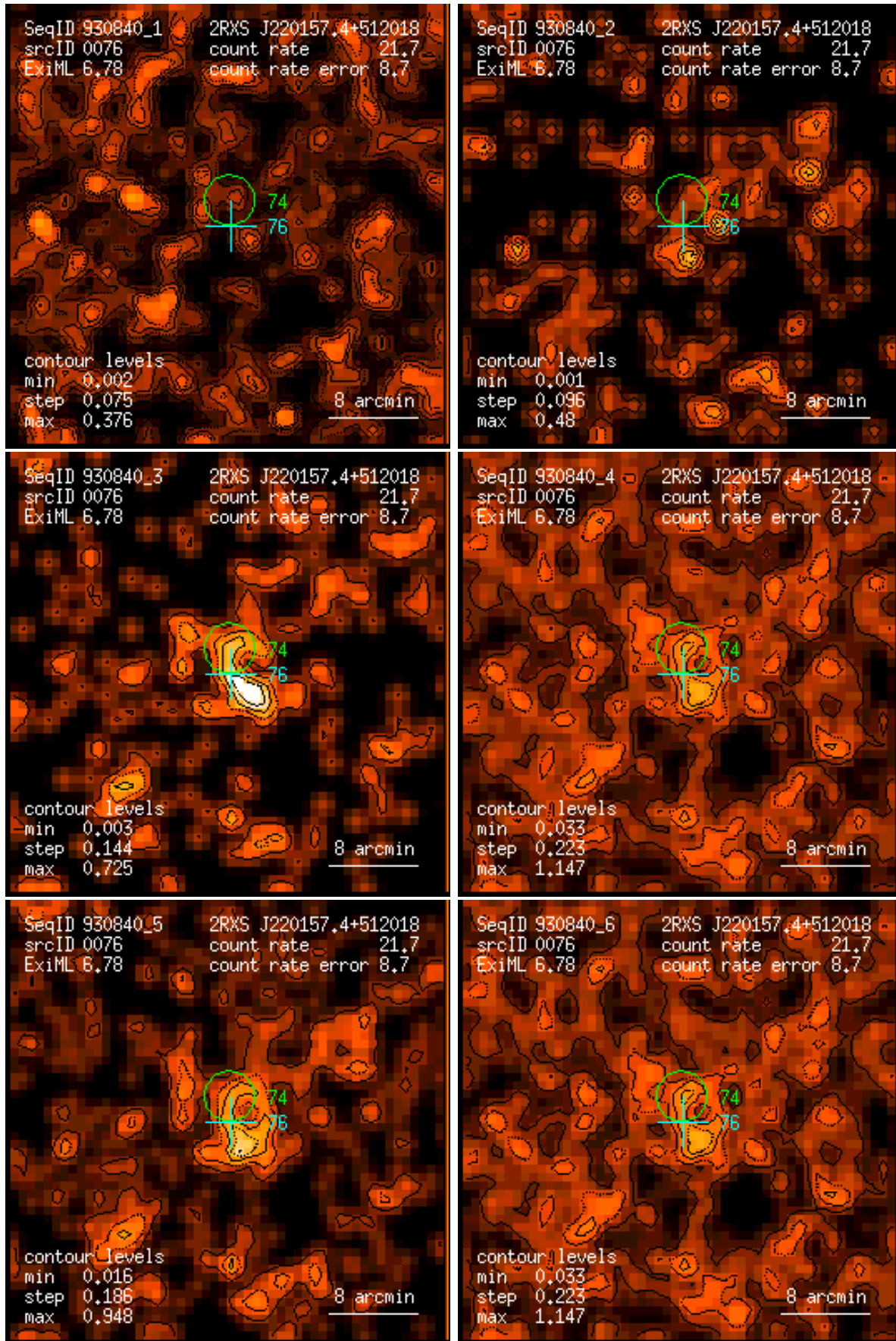
Figure 76: RASS 930840: detection 0076: band rate images, Gaussian filter: (1) PSPC channels 11 – 41, (2) 52 – 90, (3) 91 – 201, (4) 11 – 235, (5) 52 – 201, (6) 11 – 201. Broad band rates in counts/ks. Band rate contour levels in counts/ks/arcmin 2 .
