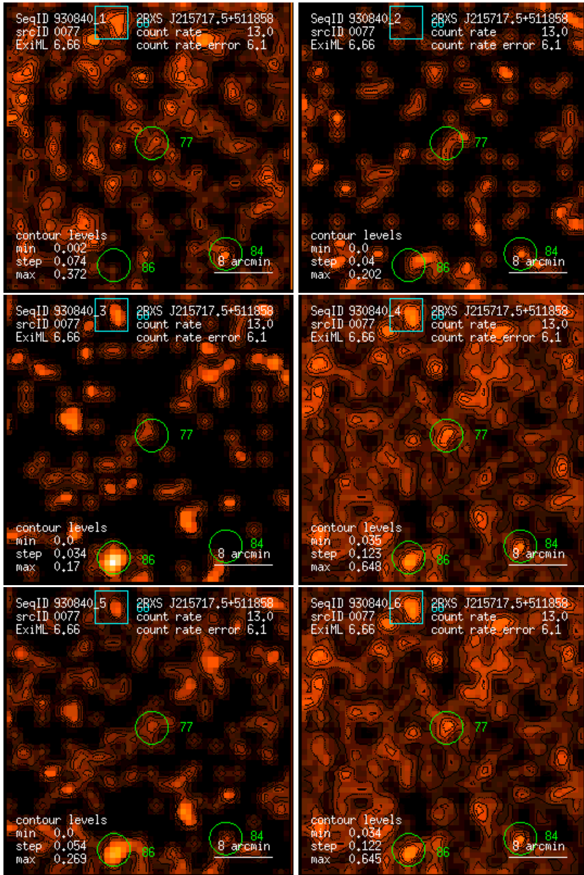
Figure 77: RASS 930840: detection 0077: band rate images, Gaussian filter: (1) PSPC channels 11 – 41, (2) 52 – 90, (3) 91 – 201, (4) 11 – 235, (5) 52 – 201, (6) 11 – 201. Broad band rates in counts/ks. Band rate contour levels in counts/ks/arcmin 2 .
