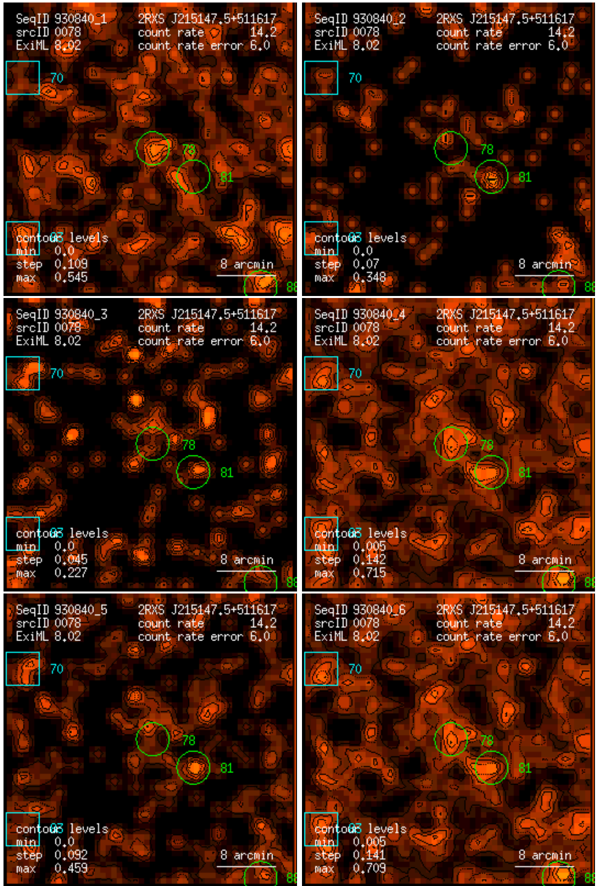
Figure 78: RASS 930840: detection 0078: band rate images, Gaussian filter: (1) PSPC channels 11 – 41, (2) 52 – 90, (3) 91 – 201, (4) 11 – 235, (5) 52 – 201, (6) 11 – 201. Broad band rates in counts/ks. Band rate contour levels in counts/ks/arcmin 2 .
