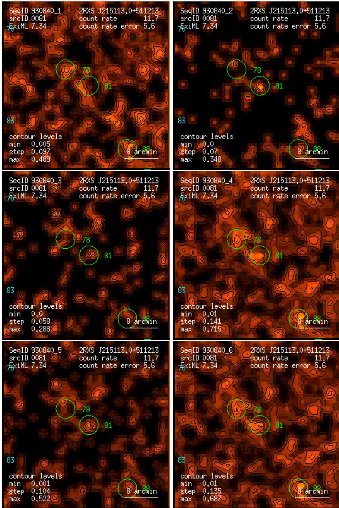
Figure 81: RASS 930840: detection 0081: band rate images, Gaussian filter: (1) PSPC channels 11 – 41, (2) 52 – 90, (3) 91 – 201, (4) 11 – 235, (5) 52 – 201, (6) 11 – 201. Broad band rates in counts/ks. Band rate contour levels in counts/ks/arcmin 2 .
