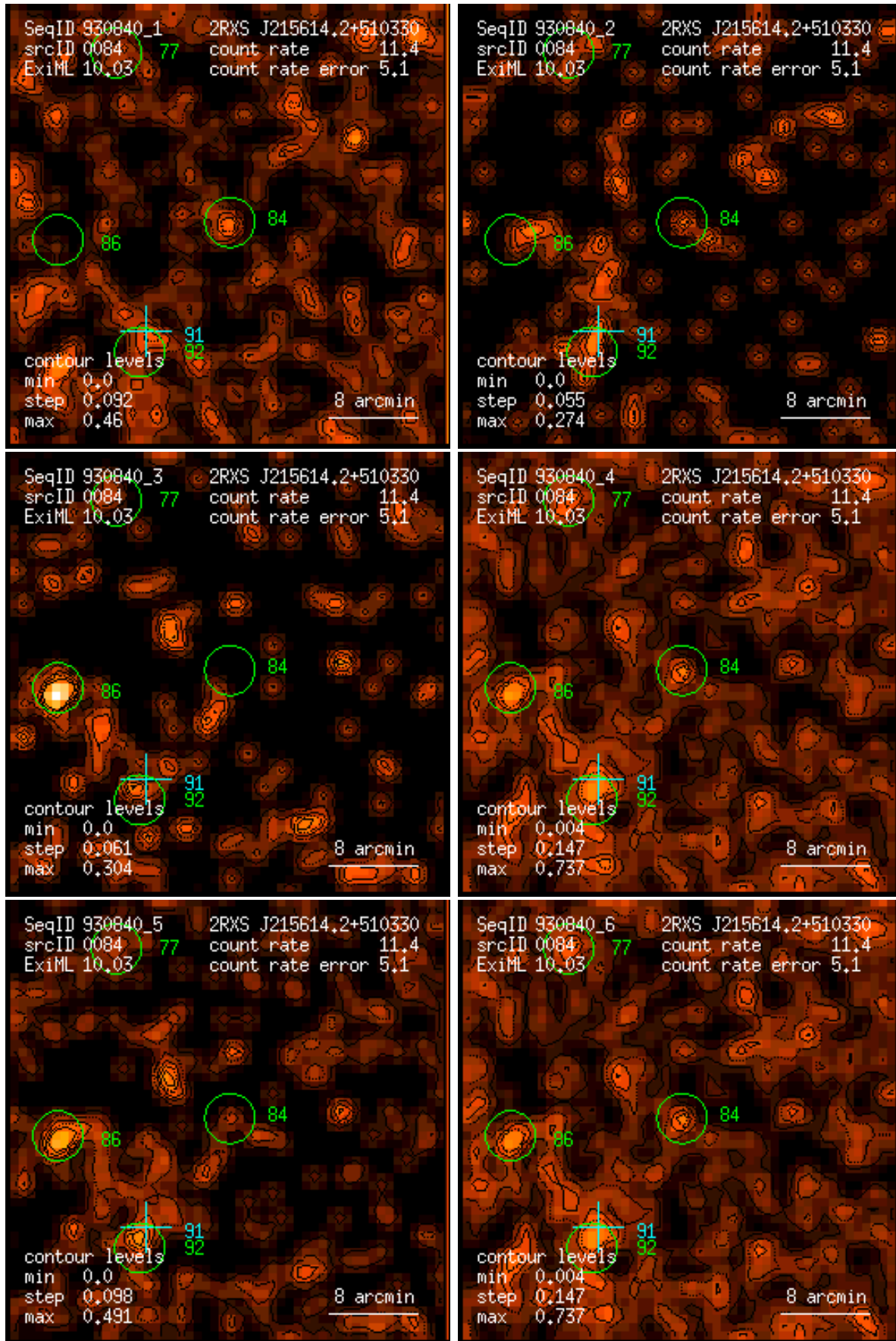
Figure 84: RASS 930840: detection 0084: band rate images, Gaussian filter: (1) PSPC channels 11 – 41, (2) 52 – 90, (3) 91 – 201, (4) 11 – 235, (5) 52 – 201, (6) 11 – 201. Broad band rates in counts/ks. Band rate contour levels in counts/ks/arcmin 2 .
