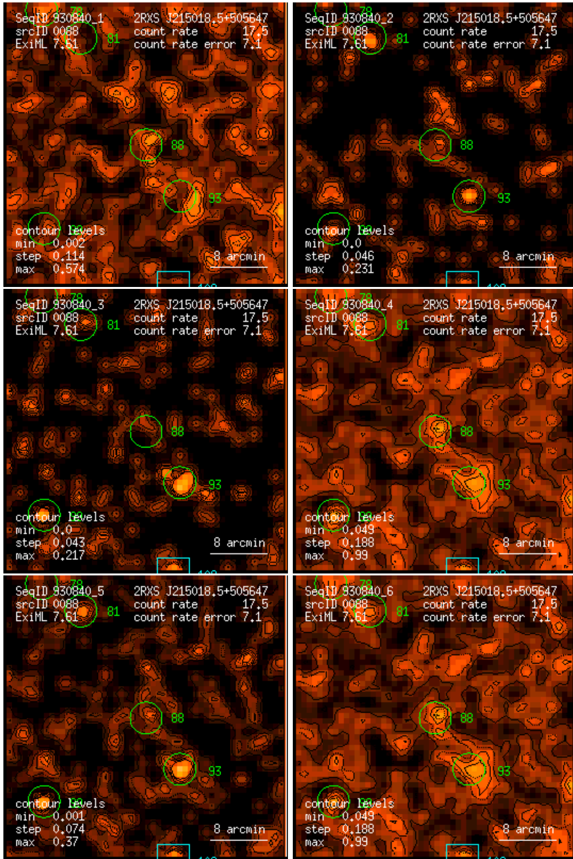
Figure 88: RASS 930840: detection 0088: band rate images, Gaussian filter: (1) PSPC channels 11 – 41, (2) 52 – 90, (3) 91 – 201, (4) 11 – 235, (5) 52 – 201, (6) 11 – 201. Broad band rates in counts/ks. Band rate contour levels in counts/ks/arcmin 2 .
