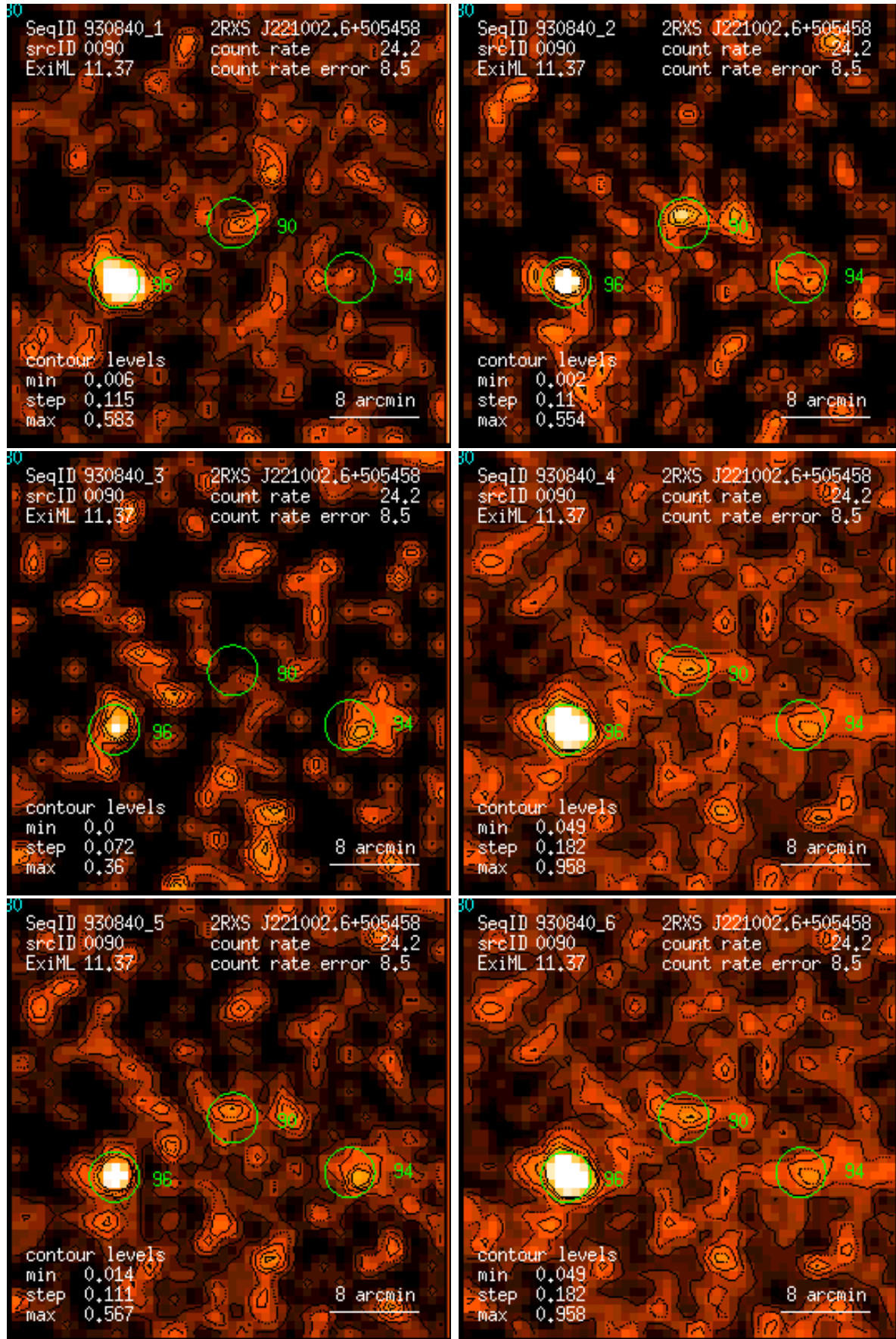
Figure 90: RASS 930840: detection 0090: band rate images, Gaussian filter: (1) PSPC channels 11 – 41, (2) 52 – 90, (3) 91 – 201, (4) 11 – 235, (5) 52 – 201, (6) 11 – 201. Broad band rates in counts/ks. Band rate contour levels in counts/ks/arcmin 2 .
