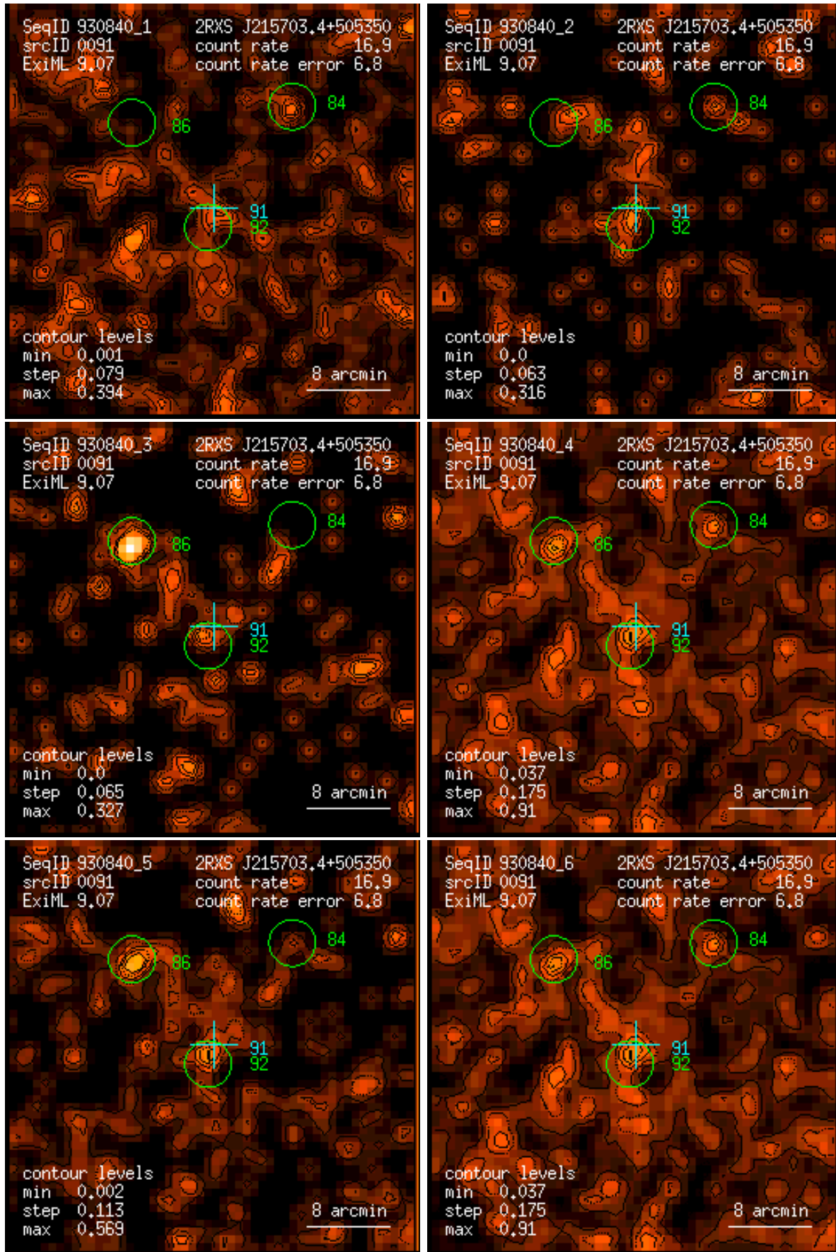
Figure 91: RASS 930840: detection 0091: band rate images, Gaussian filter: (1) PSPC channels 11 – 41, (2) 52 – 90, (3) 91 – 201, (4) 11 – 235, (5) 52 – 201, (6) 11 – 201. Broad band rates in counts/ks. Band rate contour levels in counts/ks/arcmin 2 .
