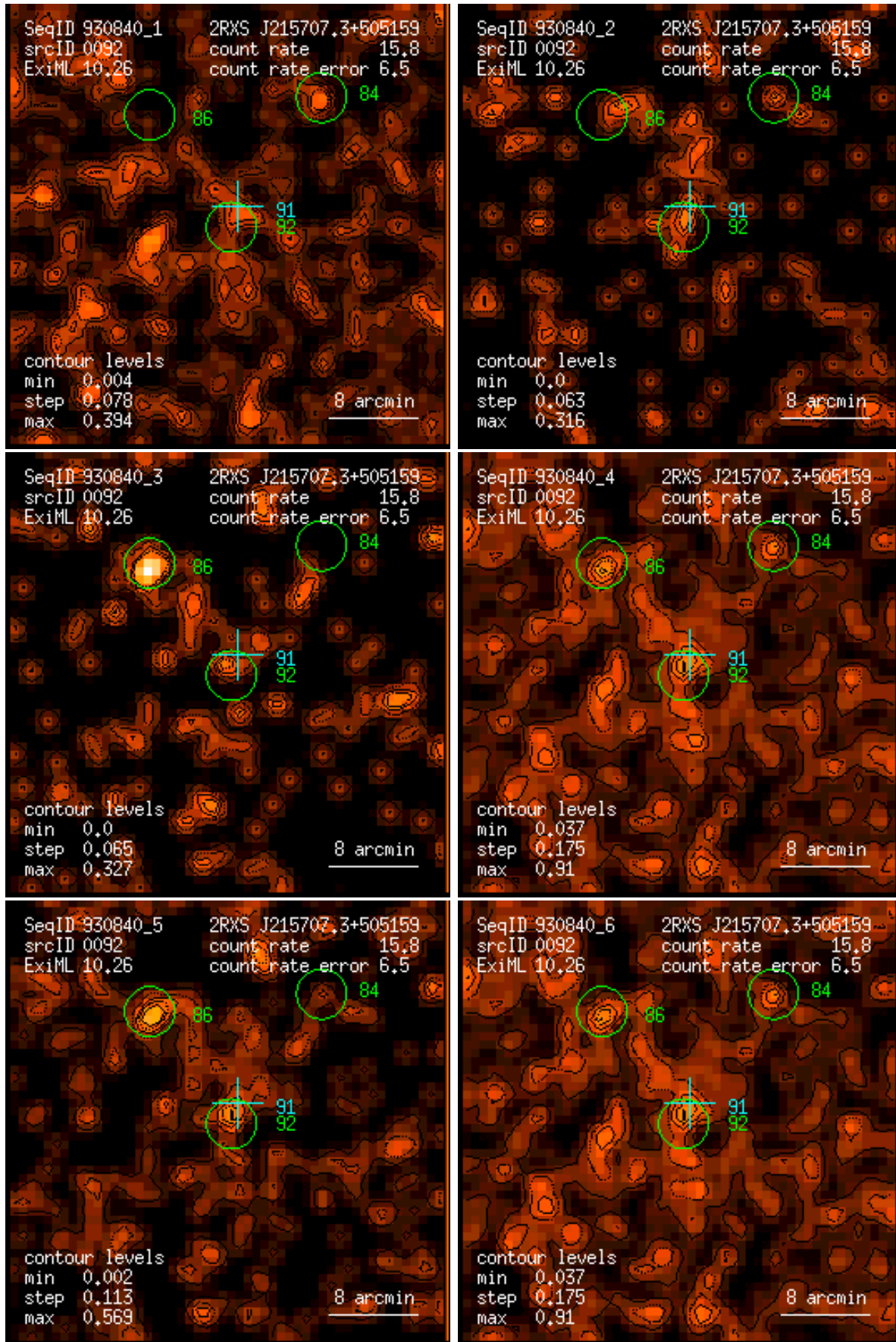
Figure 92: RASS 930840: detection 0092: band rate images, Gaussian filter: (1) PSPC channels 11 – 41, (2) 52 – 90, (3) 91 – 201, (4) 11 – 235, (5) 52 – 201, (6) 11 – 201. Broad band rates in counts/ks. Band rate contour levels in counts/ks/arcmin 2 .
