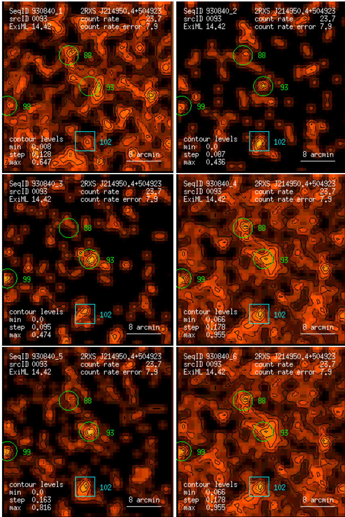
Figure 93: RASS 930840: detection 0093: band rate images, Gaussian filter: (1) PSPC channels 11 – 41, (2) 52 – 90, (3) 91 – 201, (4) 11 – 235, (5) 52 – 201, (6) 11 – 201. Broad band rates in counts/ks. Band rate contour levels in counts/ks/arcmin 2 .
