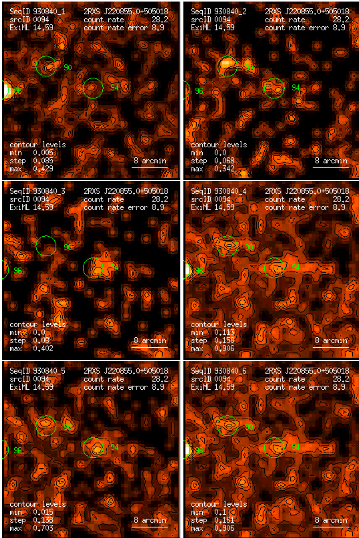
Figure 94: RASS 930840: detection 0094: band rate images, Gaussian filter: (1) PSPC channels 11 – 41, (2) 52 – 90, (3) 91 – 201, (4) 11 – 235, (5) 52 – 201, (6) 11 – 201. Broad band rates in counts/ks. Band rate contour levels in counts/ks/arcmin 2 .
