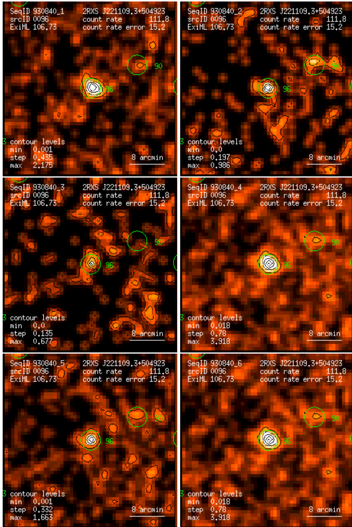
Figure 96: RASS 930840: detection 0096: band rate images, Gaussian filter: (1) PSPC channels 11 – 41, (2) 52 – 90, (3) 91 – 201, (4) 11 – 235, (5) 52 – 201, (6) 11 – 201. Broad band rates in counts/ks. Band rate contour levels in counts/ks/arcmin 2 .
