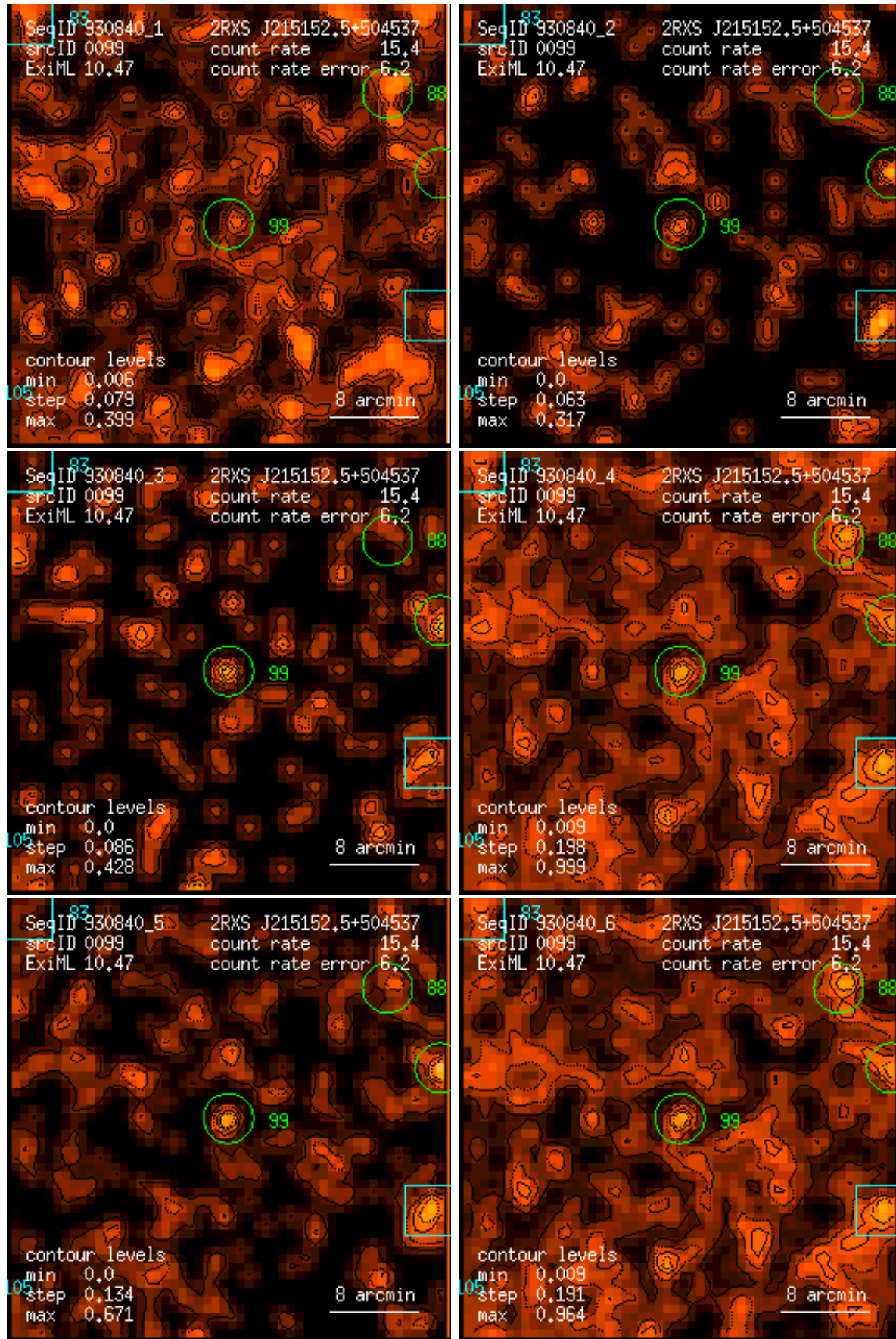
Figure 99: RASS 930840: detection 0099: band rate images, Gaussian filter: (1) PSPC channels 11 – 41, (2) 52 – 90, (3) 91 – 201, (4) 11 – 235, (5) 52 – 201, (6) 11 – 201. Broad band rates in counts/ks. Band rate contour levels in counts/ks/arcmin 2 .
