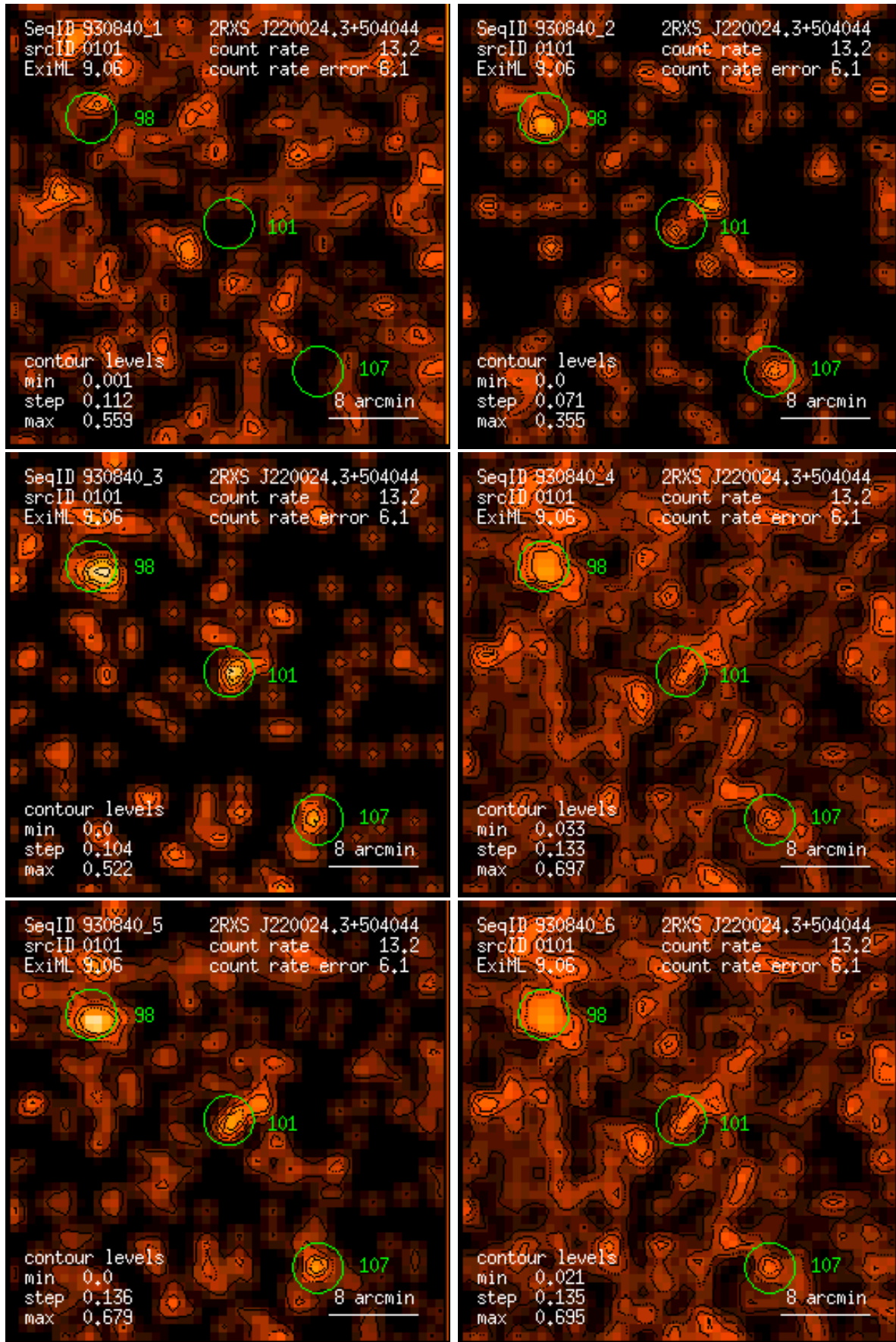
Figure 101: RASS 930840: detection 0101: band rate images, Gaussian filter: (1) PSPC channels 11 – 41, (2) 52 – 90, (3) 91 – 201, (4) 11 – 235, (5) 52 – 201, (6) 11 – 201. Broad band rates in counts/ks. Band rate contour levels in counts/ks/arcmin 2 .
