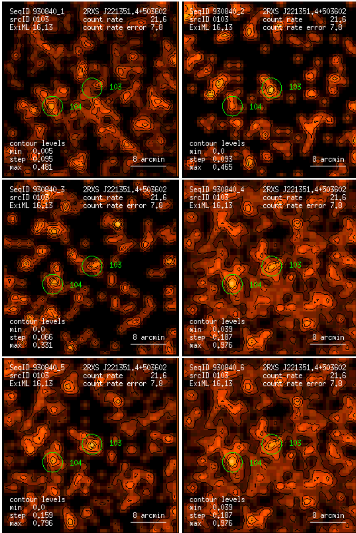
Figure 103: RASS 930840: detection 0103: band rate images, Gaussian filter: (1) PSPC channels 11 – 41, (2) 52 – 90, (3) 91 – 201, (4) 11 – 235, (5) 52 – 201, (6) 11 – 201. Broad band rates in counts/ks. Band rate contour levels in counts/ks/arcmin 2 .
