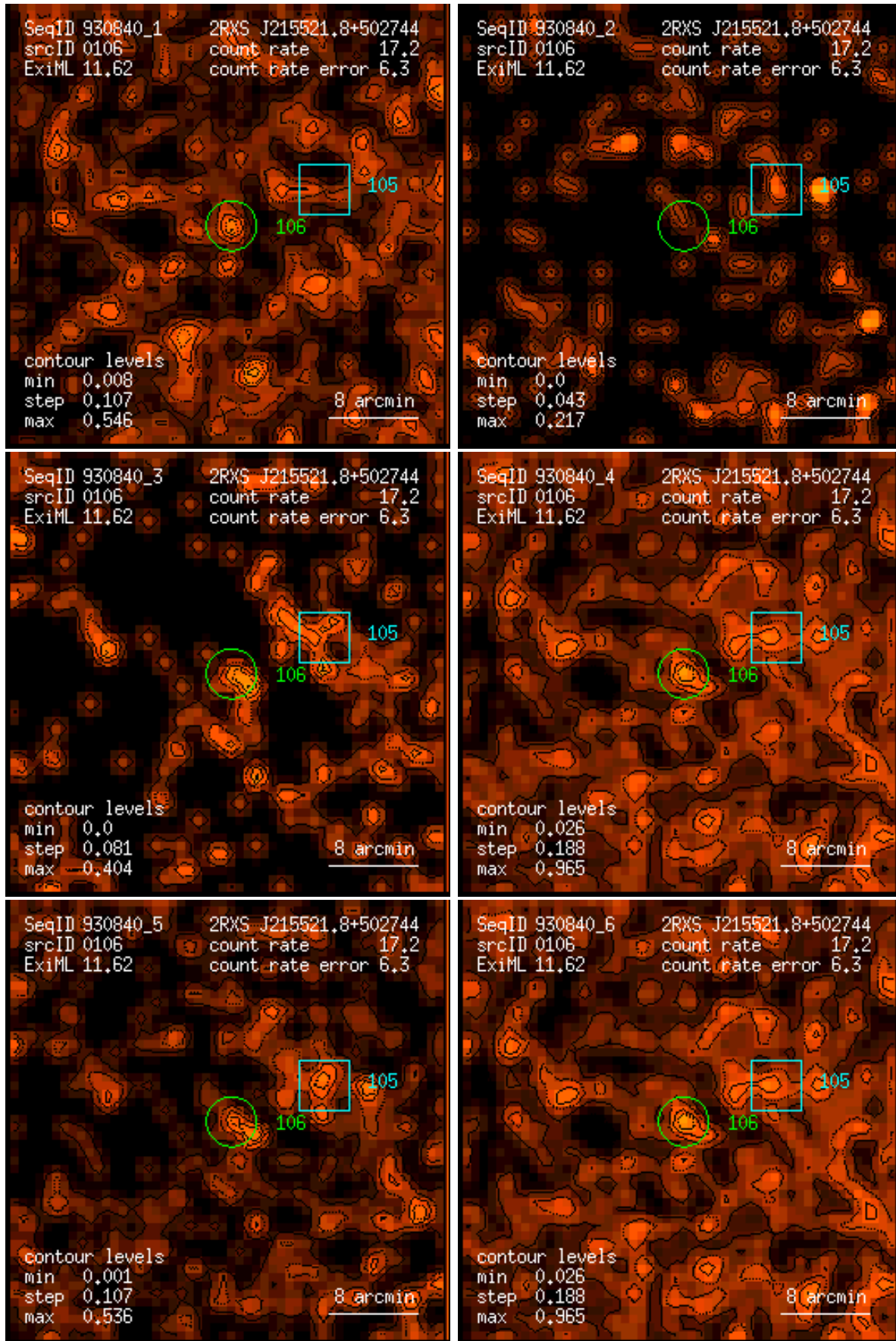
Figure 106: RASS 930840: detection 0106: band rate images, Gaussian filter: (1) PSPC channels 11 – 41, (2) 52 – 90, (3) 91 – 201, (4) 11 – 235, (5) 52 – 201, (6) 11 – 201. Broad band rates in counts/ks. Band rate contour levels in counts/ks/arcmin 2 .
