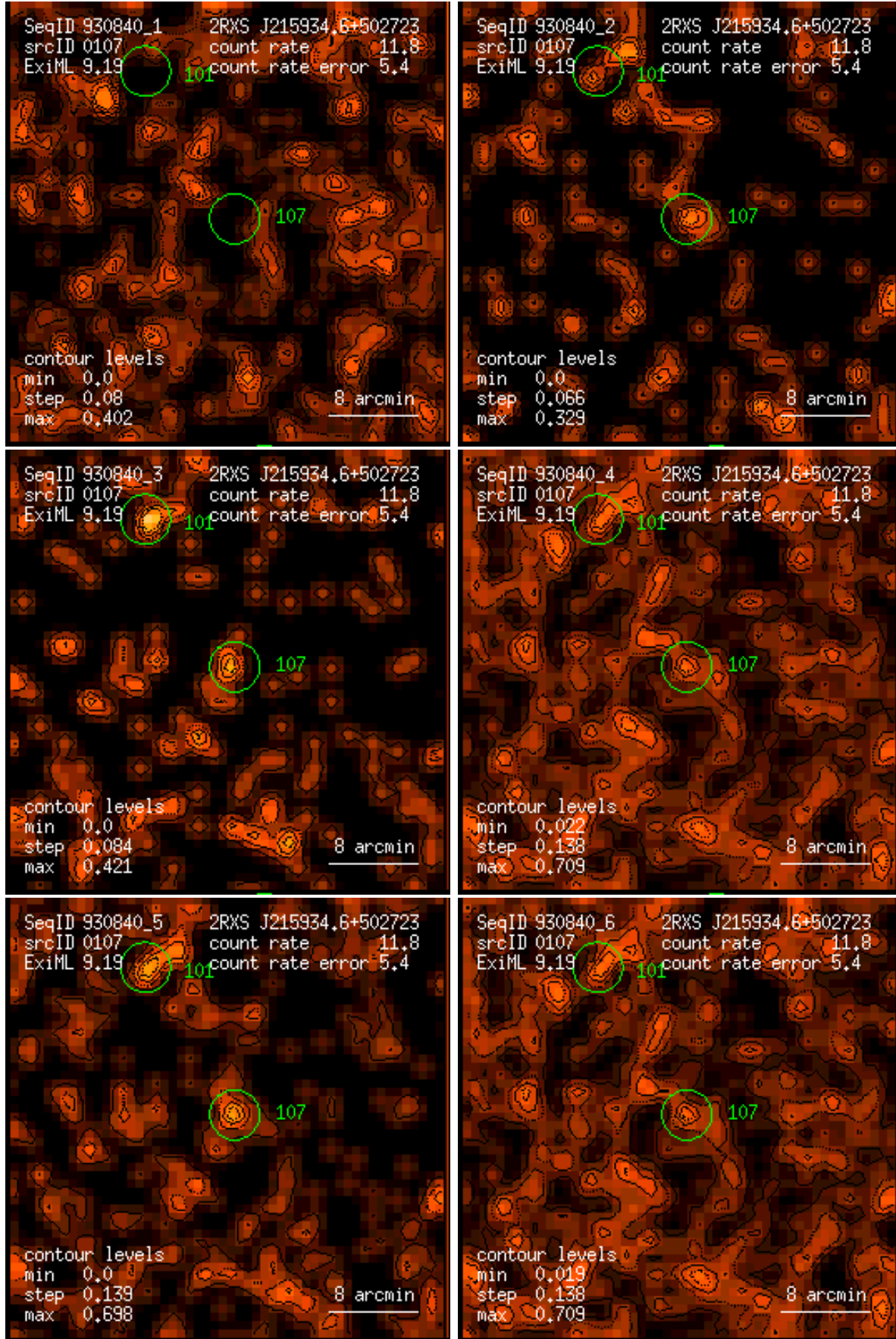
Figure 107: RASS 930840: detection 0107: band rate images, Gaussian filter: (1) PSPC channels 11 – 41, (2) 52 – 90, (3) 91 – 201, (4) 11 – 235, (5) 52 – 201, (6) 11 – 201. Broad band rates in counts/ks. Band rate contour levels in counts/ks/arcmin 2 .
