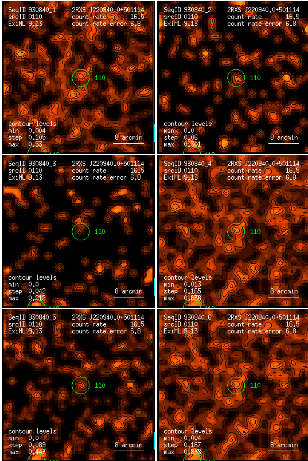
Figure 110: RASS 930840: detection 0110: band rate images, Gaussian filter: (1) PSPC channels 11 – 41, (2) 52 – 90, (3) 91 – 201, (4) 11 – 235, (5) 52 – 201, (6) 11 – 201. Broad band rates in counts/ks. Band rate contour levels in counts/ks/arcmin 2 .
