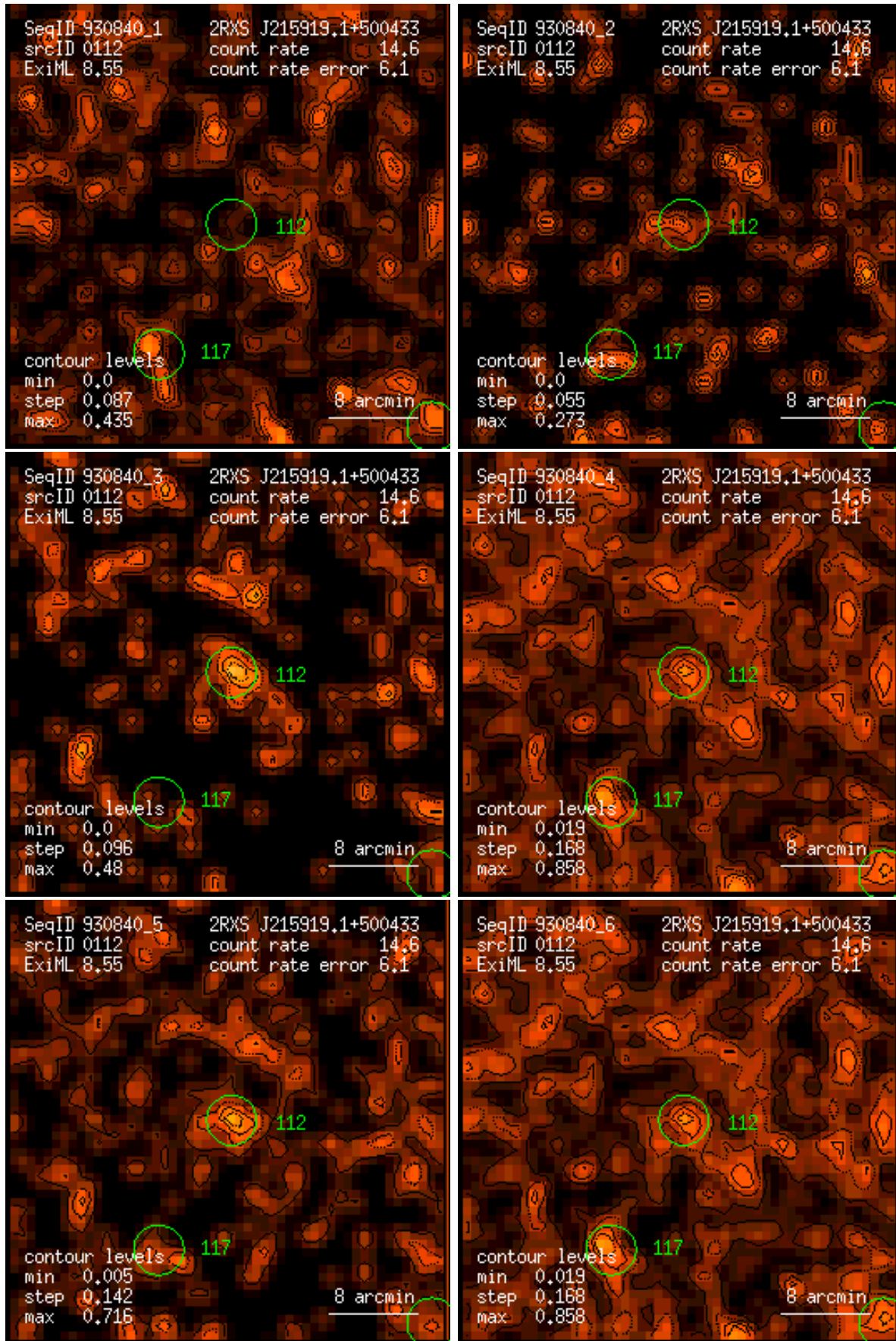
Figure 112: RASS 930840: detection 0112: band rate images, Gaussian filter: (1) PSPC channels 11 – 41, (2) 52 – 90, (3) 91 – 201, (4) 11 – 235, (5) 52 – 201, (6) 11 – 201. Broad band rates in counts/ks. Band rate contour levels in counts/ks/arcmin 2 .
