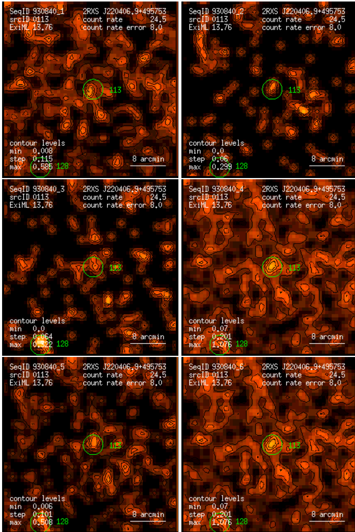
Figure 113: RASS 930840: detection 0113: band rate images, Gaussian filter: (1) PSPC channels 11 – 41, (2) 52 – 90, (3) 91 – 201, (4) 11 – 235, (5) 52 – 201, (6) 11 – 201. Broad band rates in counts/ks. Band rate contour levels in counts/ks/arcmin 2 .
