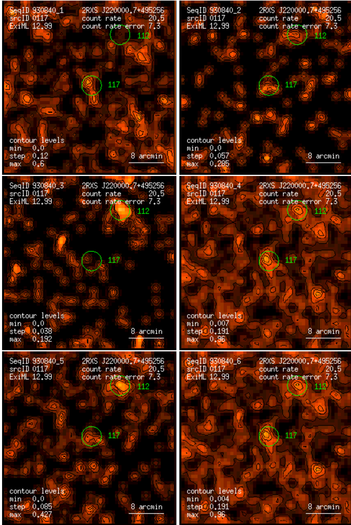
Figure 117: RASS 930840: detection 0117: band rate images, Gaussian filter: (1) PSPC channels 11 – 41, (2) 52 – 90, (3) 91 – 201, (4) 11 – 235, (5) 52 – 201, (6) 11 – 201. Broad band rates in counts/ks. Band rate contour levels in counts/ks/arcmin 2 .
