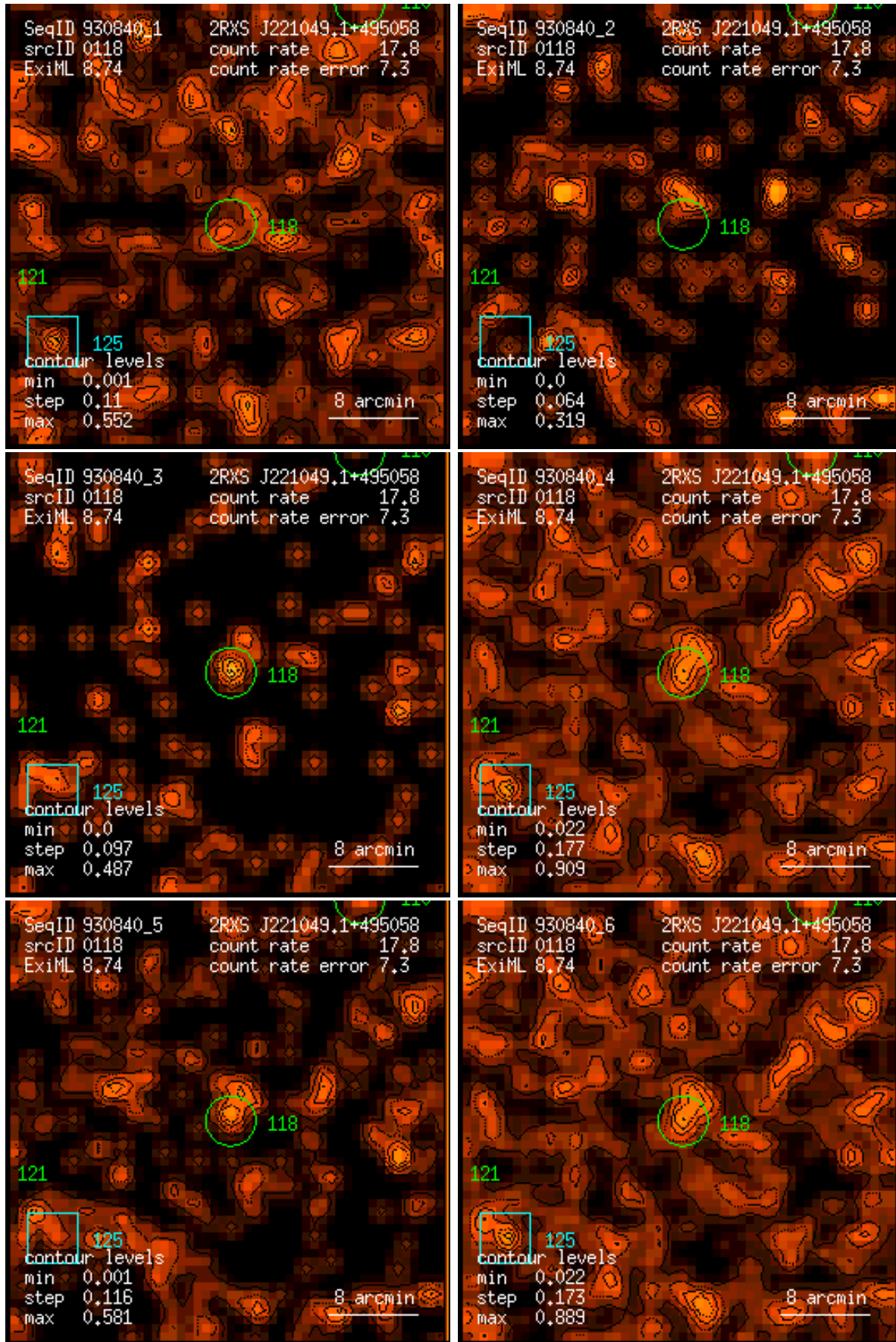
Figure 118: RASS 930840: detection 0118: band rate images, Gaussian filter: (1) PSPC channels 11 – 41, (2) 52 – 90, (3) 91 – 201, (4) 11 – 235, (5) 52 – 201, (6) 11 – 201. Broad band rates in counts/ks. Band rate contour levels in counts/ks/arcmin 2 .
