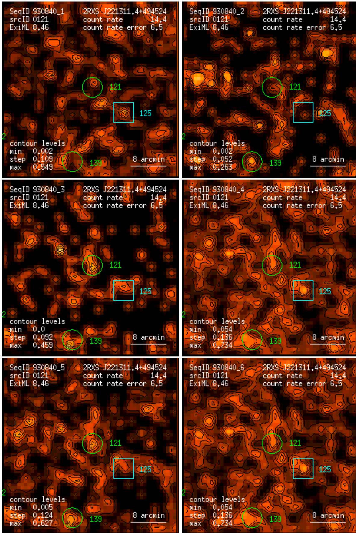
Figure 121: RASS 930840: detection 0121: band rate images, Gaussian filter: (1) PSPC channels 11 – 41, (2) 52 – 90, (3) 91 – 201, (4) 11 – 235, (5) 52 – 201, (6) 11 – 201. Broad band rates in counts/ks. Band rate contour levels in counts/ks/arcmin 2 .
