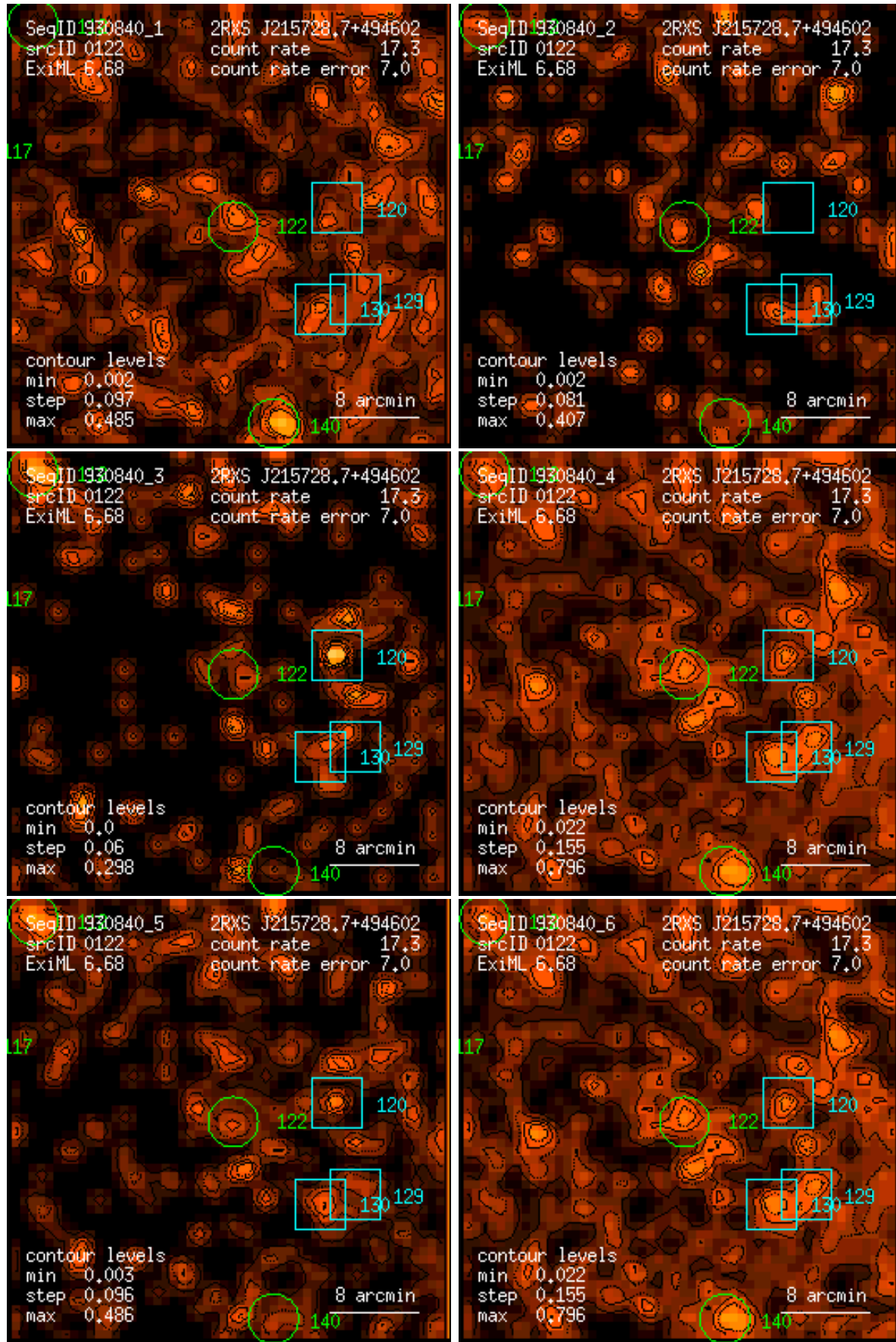
Figure 122: RASS 930840: detection 0122: band rate images, Gaussian filter: (1) PSPC channels 11 – 41, (2) 52 – 90, (3) 91 – 201, (4) 11 – 235, (5) 52 – 201, (6) 11 – 201. Broad band rates in counts/ks. Band rate contour levels in counts/ks/arcmin 2 .
