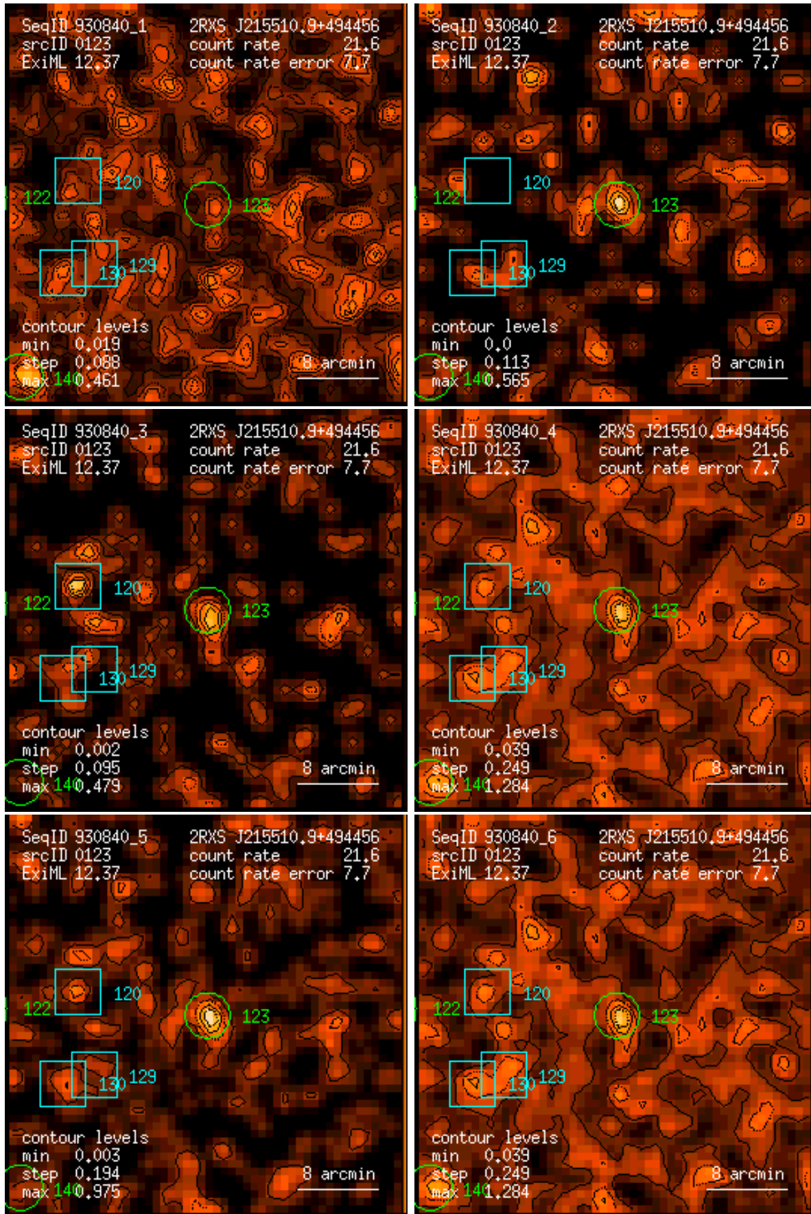
Figure 123: RASS 930840: detection 0123: band rate images, Gaussian filter: (1) PSPC channels 11 – 41, (2) 52 – 90, (3) 91 – 201, (4) 11 – 235, (5) 52 – 201, (6) 11 – 201. Broad band rates in counts/ks. Band rate contour levels in counts/ks/arcmin 2 .
