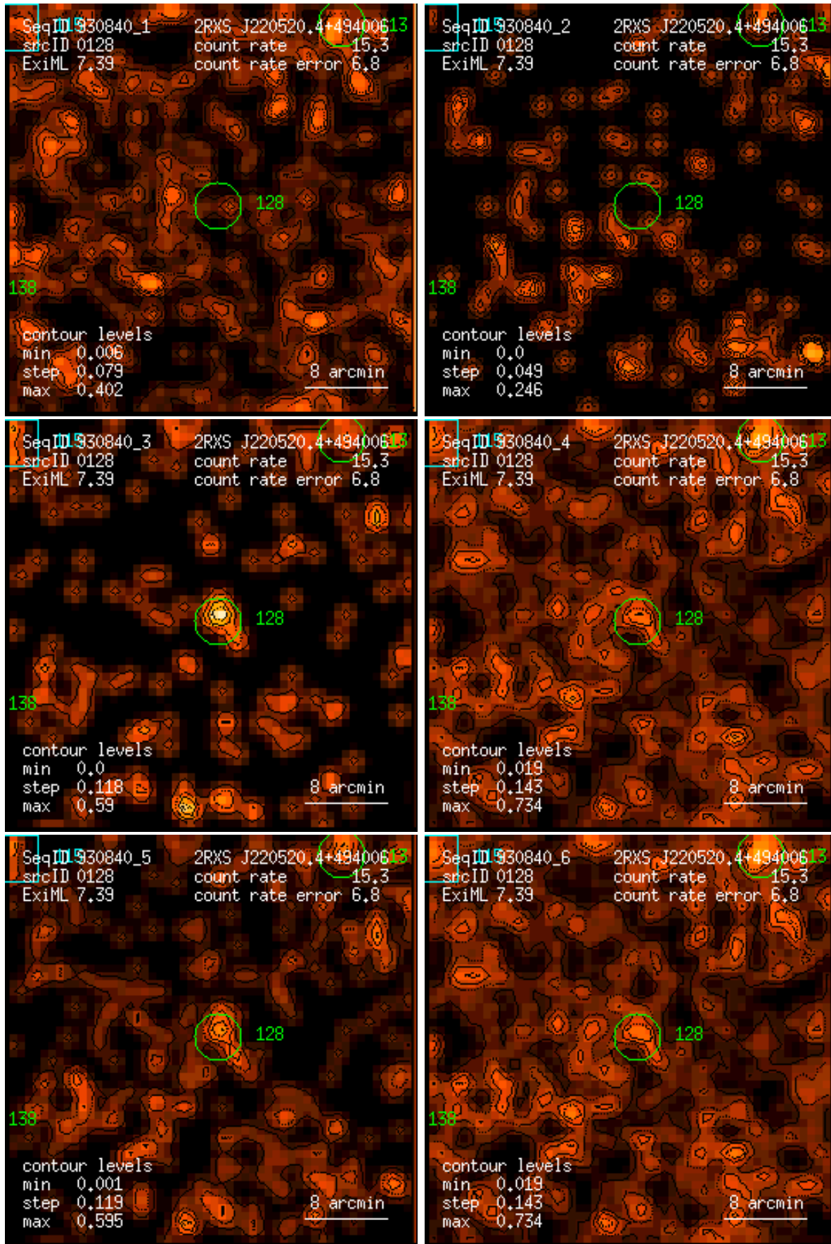
Figure 128: RASS 930840: detection 0128: band rate images, Gaussian filter: (1) PSPC channels 11 – 41, (2) 52 – 90, (3) 91 – 201, (4) 11 – 235, (5) 52 – 201, (6) 11 – 201. Broad band rates in counts/ks. Band rate contour levels in counts/ks/arcmin 2 .
