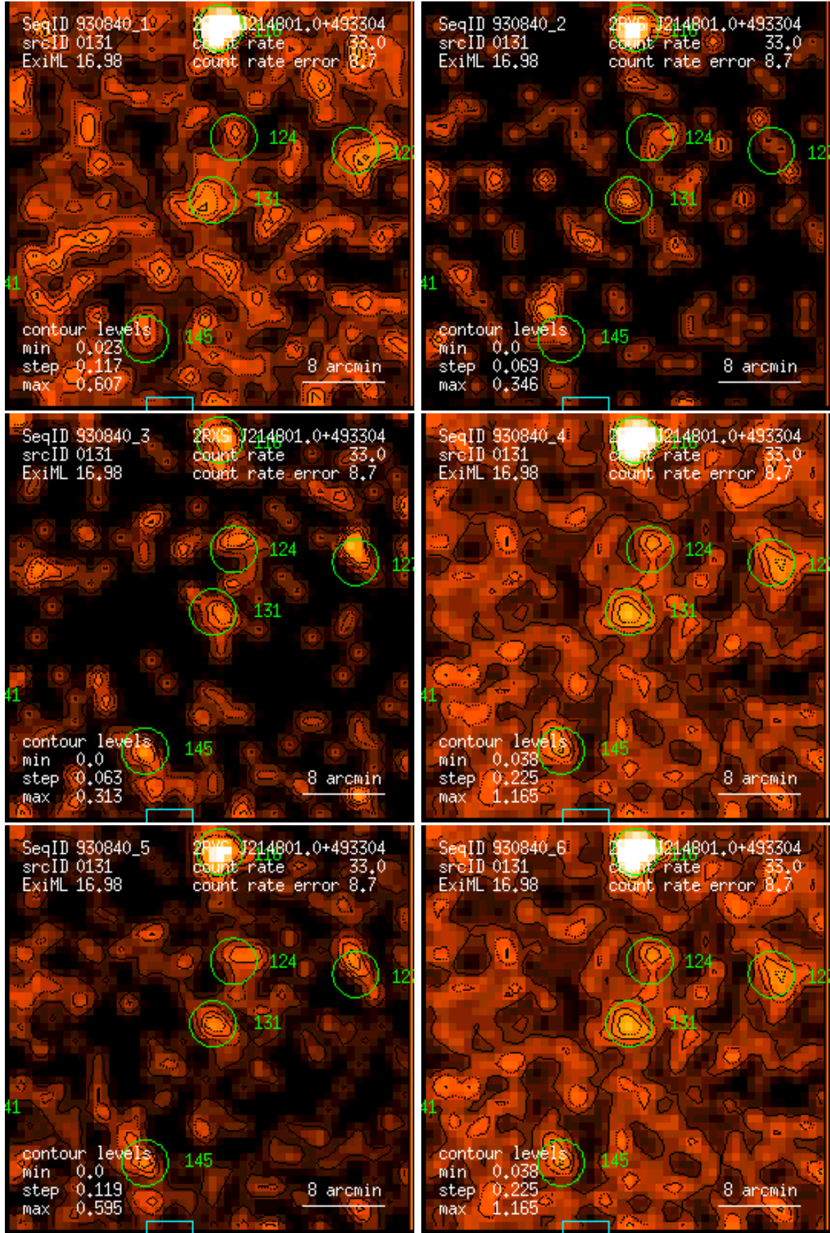
Figure 131: RASS 930840: detection 0131: band rate images, Gaussian filter: (1) PSPC channels 11 – 41, (2) 52 – 90, (3) 91 – 201, (4) 11 – 235, (5) 52 – 201, (6) 11 – 201. Broad band rates in counts/ks. Band rate contour levels in counts/ks/arcmin 2 .
