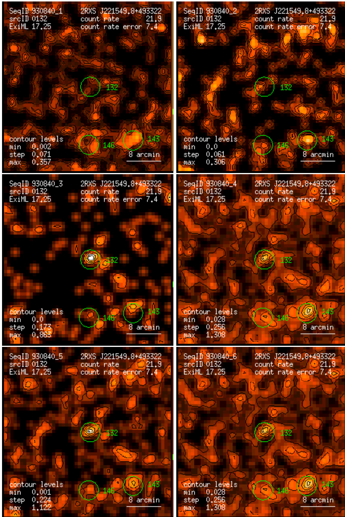
Figure 132: RASS 930840: detection 0132: band rate images, Gaussian filter: (1) PSPC channels 11 – 41, (2) 52 – 90, (3) 91 – 201, (4) 11 – 235, (5) 52 – 201, (6) 11 – 201. Broad band rates in counts/ks. Band rate contour levels in counts/ks/arcmin 2 .
