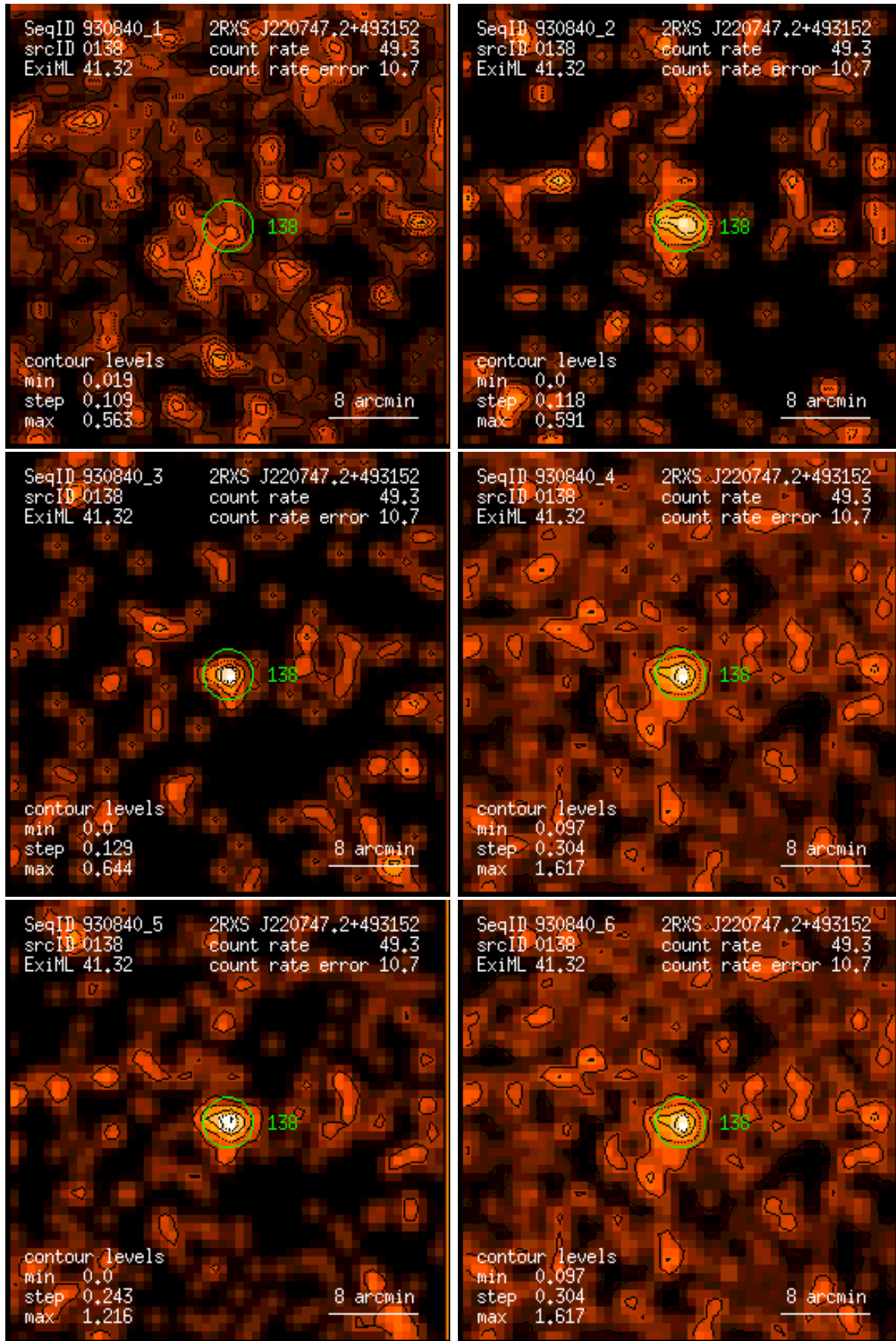
Figure 138: RASS 930840: detection 0138: band rate images, Gaussian filter: (1) PSPC channels 11 – 41, (2) 52 – 90, (3) 91 – 201, (4) 11 – 235, (5) 52 – 201, (6) 11 – 201. Broad band rates in counts/ks. Band rate contour levels in counts/ks/arcmin 2 .
