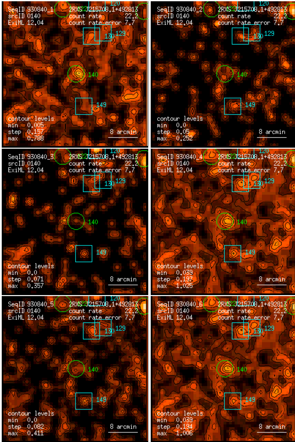
Figure 140: RASS 930840: detection 0140: band rate images, Gaussian filter: (1) PSPC channels 11 – 41, (2) 52 – 90, (3) 91 – 201, (4) 11 – 235, (5) 52 – 201, (6) 11 – 201. Broad band rates in counts/ks. Band rate contour levels in counts/ks/arcmin 2 .
