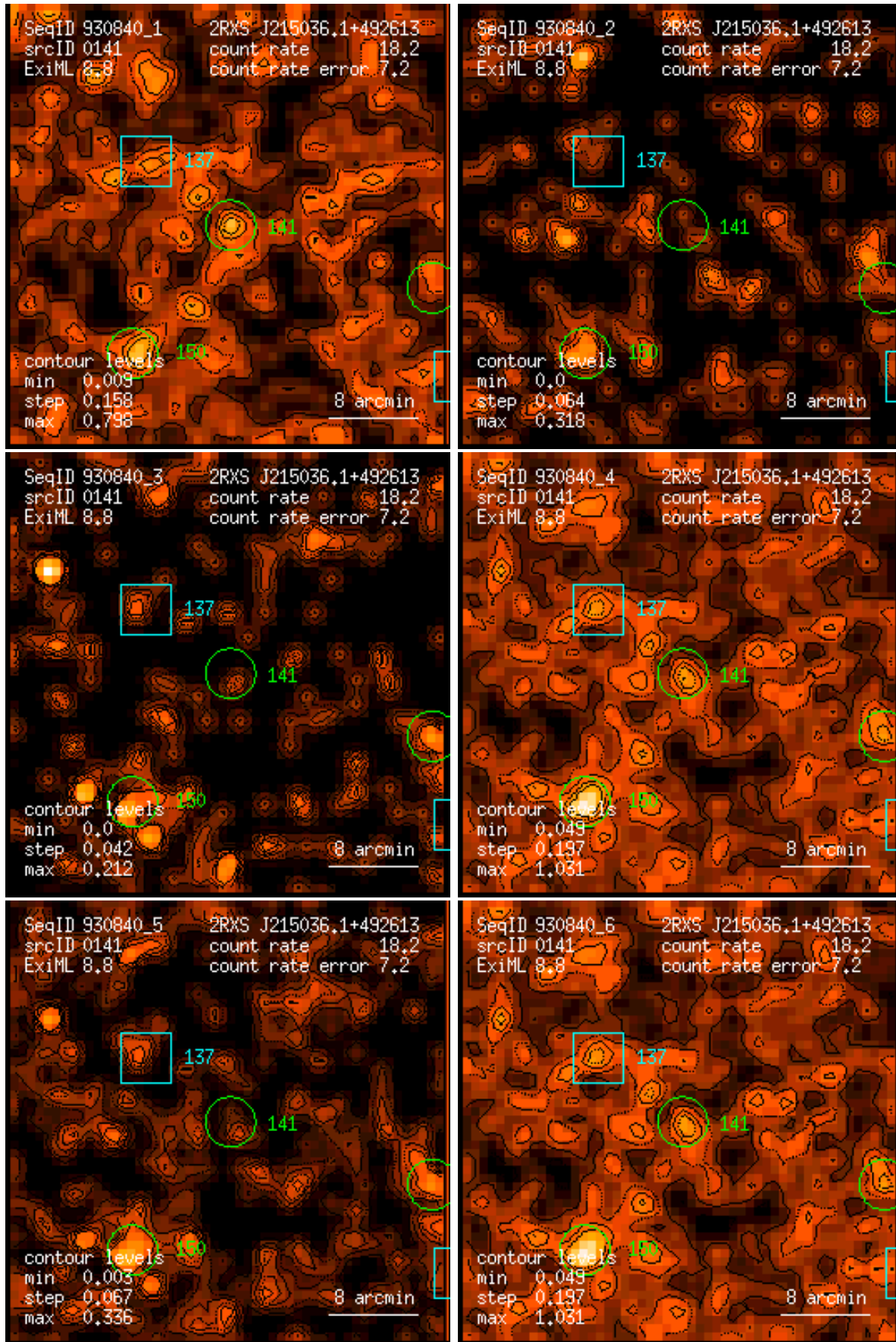
Figure 141: RASS 930840: detection 0141: band rate images, Gaussian filter: (1) PSPC channels 11 – 41, (2) 52 – 90, (3) 91 – 201, (4) 11 – 235, (5) 52 – 201, (6) 11 – 201. Broad band rates in counts/ks. Band rate contour levels in counts/ks/arcmin 2 .
