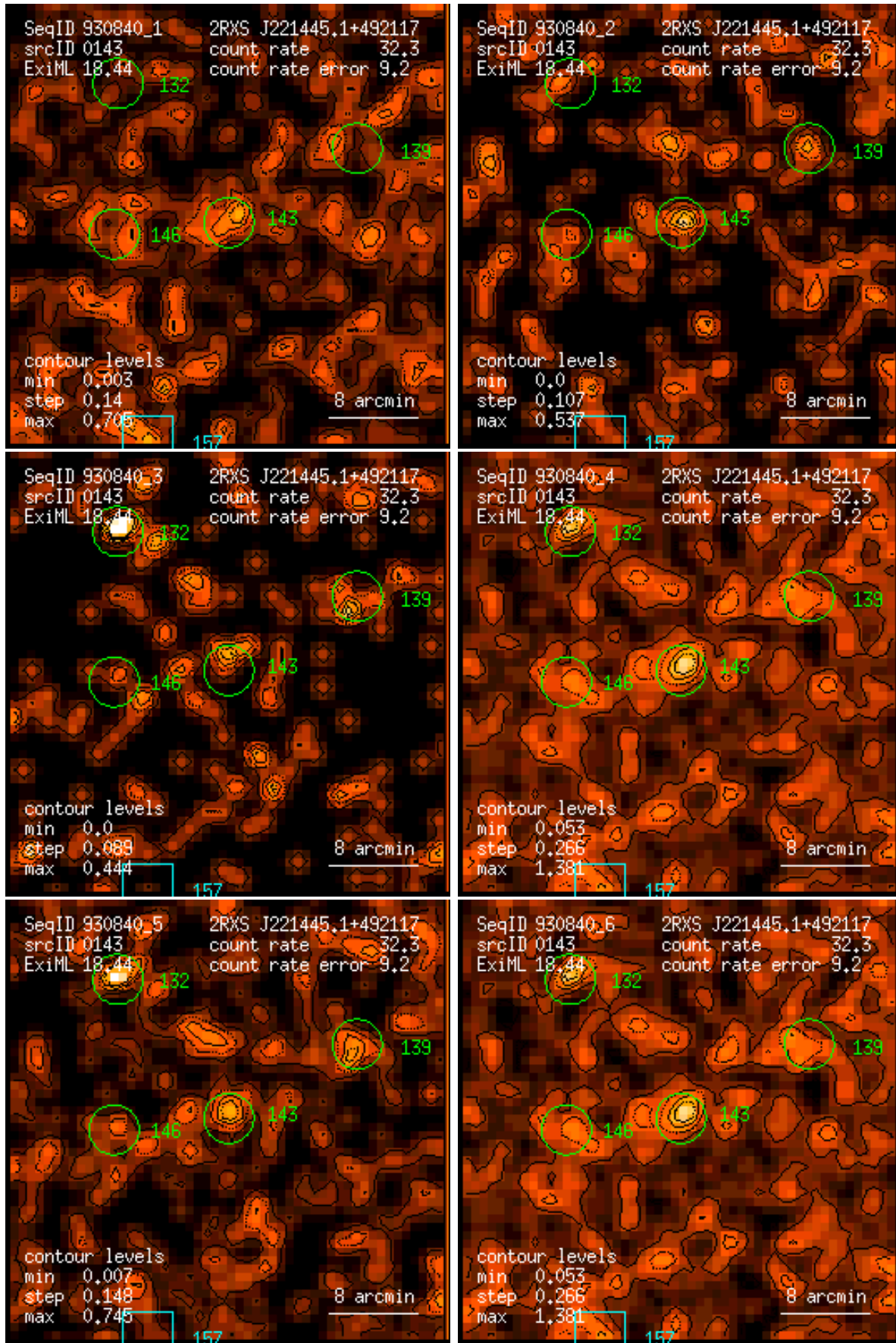
Figure 143: RASS 930840: detection 0143: band rate images, Gaussian filter: (1) PSPC channels 11 – 41, (2) 52 – 90, (3) 91 – 201, (4) 11 – 235, (5) 52 – 201, (6) 11 – 201. Broad band rates in counts/ks. Band rate contour levels in counts/ks/arcmin 2 .
