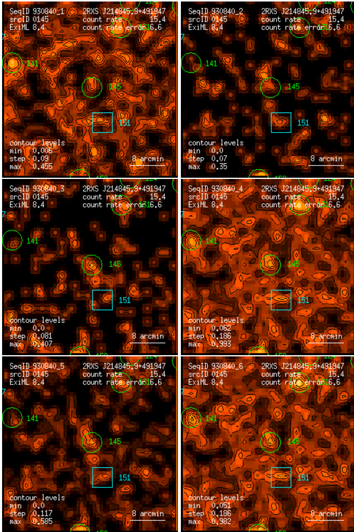
Figure 145: RASS 930840: detection 0145: band rate images, Gaussian filter: (1) PSPC channels 11 – 41, (2) 52 – 90, (3) 91 – 201, (4) 11 – 235, (5) 52 – 201, (6) 11 – 201. Broad band rates in counts/ks. Band rate contour levels in counts/ks/arcmin 2 .
