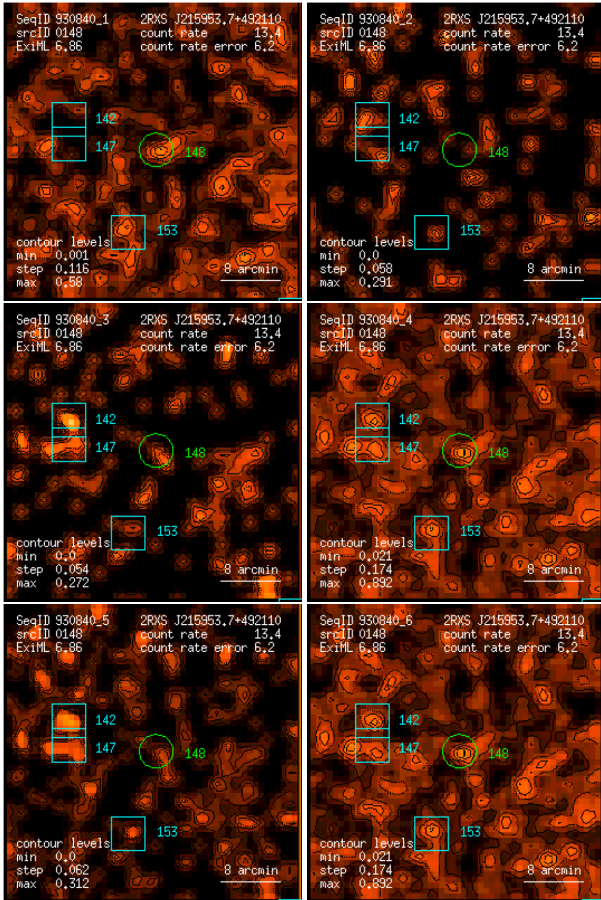
Figure 148: RASS 930840: detection 0148: band rate images, Gaussian filter: (1) PSPC channels 11 – 41, (2) 52 – 90, (3) 91 – 201, (4) 11 – 235, (5) 52 – 201, (6) 11 – 201. Broad band rates in counts/ks. Band rate contour levels in counts/ks/arcmin 2 .
