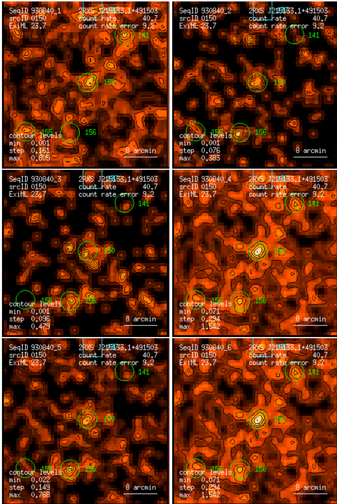
Figure 150: RASS 930840: detection 0150: band rate images, Gaussian filter: (1) PSPC channels 11 – 41, (2) 52 – 90, (3) 91 – 201, (4) 11 – 235, (5) 52 – 201, (6) 11 – 201. Broad band rates in counts/ks. Band rate contour levels in counts/ks/arcmin 2 .
