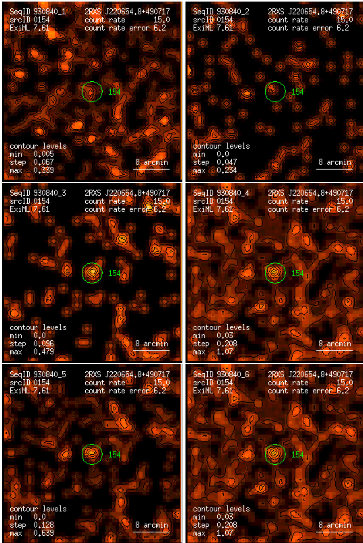
Figure 154: RASS 930840: detection 0154: band rate images, Gaussian filter: (1) PSPC channels 11 – 41, (2) 52 – 90, (3) 91 – 201, (4) 11 – 235, (5) 52 – 201, (6) 11 – 201. Broad band rates in counts/ks. Band rate contour levels in counts/ks/arcmin 2 .
