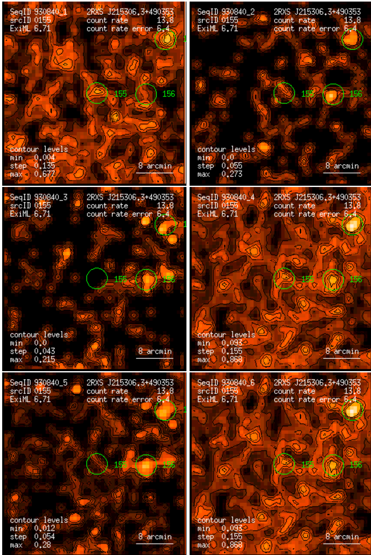
Figure 155: RASS 930840: detection 0155: band rate images, Gaussian filter: (1) PSPC channels 11 – 41, (2) 52 – 90, (3) 91 – 201, (4) 11 – 235, (5) 52 – 201, (6) 11 – 201. Broad band rates in counts/ks. Band rate contour levels in counts/ks/arcmin 2 .
