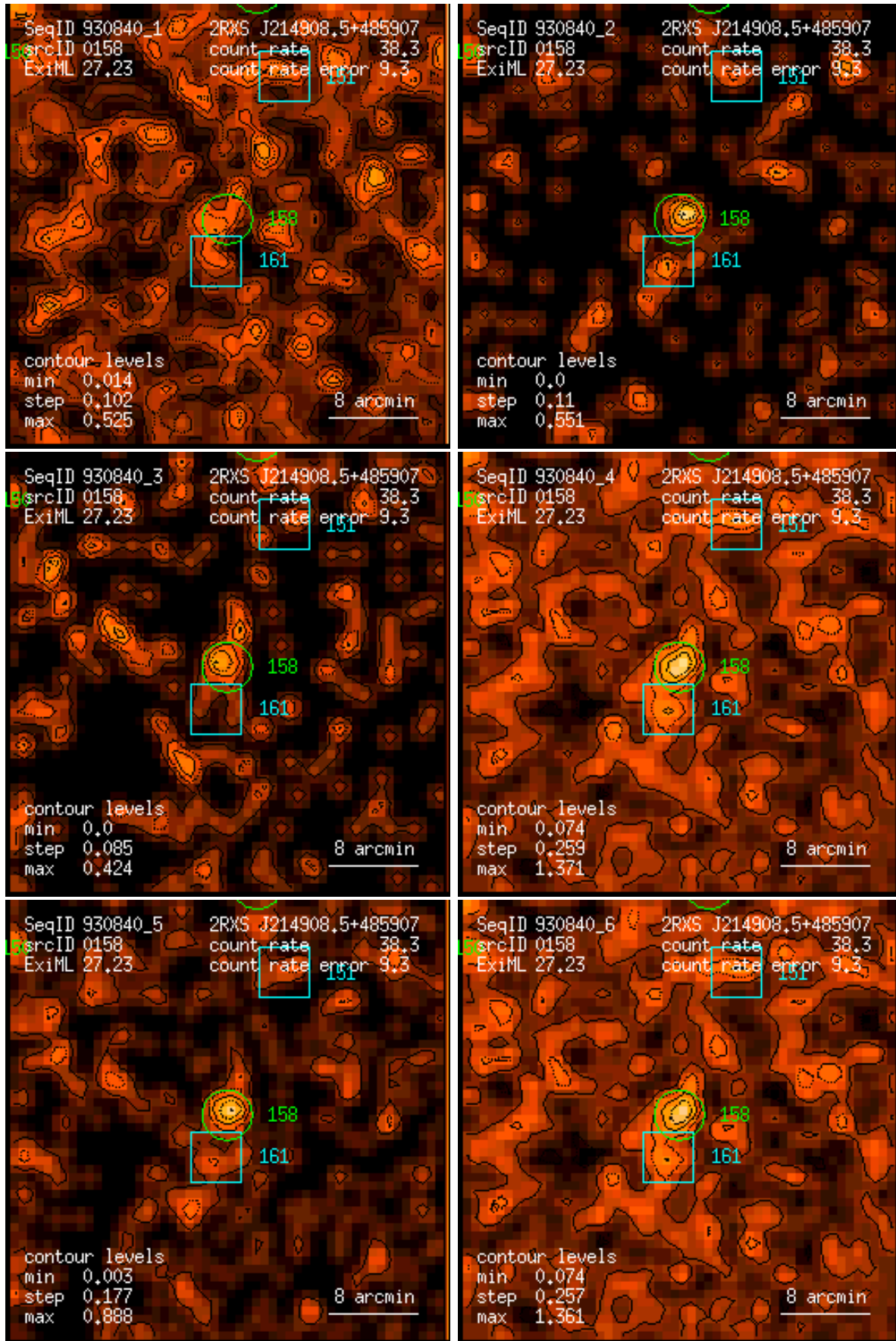
Figure 158: RASS 930840: detection 0158: band rate images, Gaussian filter: (1) PSPC channels 11 – 41, (2) 52 – 90, (3) 91 – 201, (4) 11 – 235, (5) 52 – 201, (6) 11 – 201. Broad band rates in counts/ks. Band rate contour levels in counts/ks/arcmin 2 .
