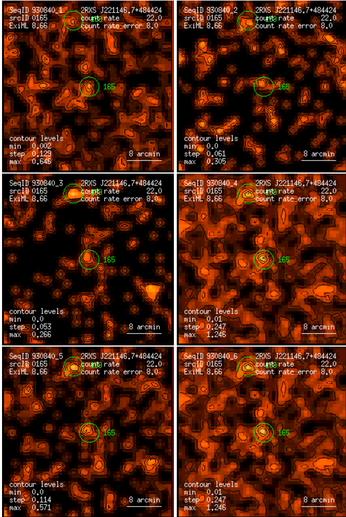
Figure 165: RASS 930840: detection 0165: band rate images, Gaussian filter: (1) PSPC channels 11 – 41, (2) 52 – 90, (3) 91 – 201, (4) 11 – 235, (5) 52 – 201, (6) 11 – 201. Broad band rates in counts/ks. Band rate contour levels in counts/ks/arcmin 2 .
