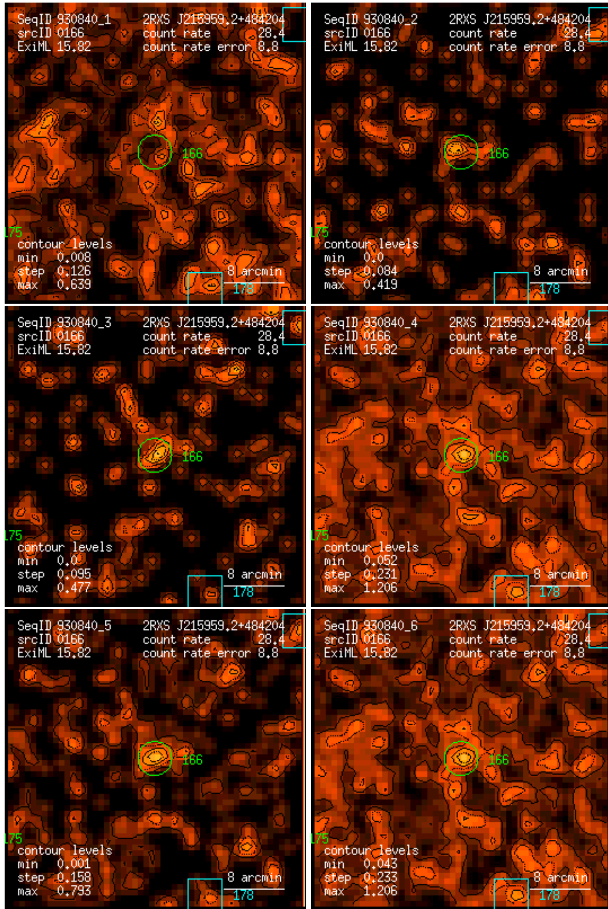
Figure 166: RASS 930840: detection 0166: band rate images, Gaussian filter: (1) PSPC channels 11 – 41, (2) 52 – 90, (3) 91 – 201, (4) 11 – 235, (5) 52 – 201, (6) 11 – 201. Broad band rates in counts/ks. Band rate contour levels in counts/ks/arcmin 2 .
